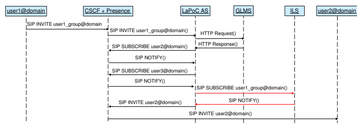
Fig. 4. Simplified LaPoC session establishment with groupInRange filters.
