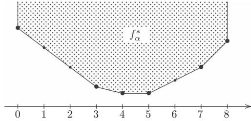
FIG. 2. Typical set f_\alpha^* , with n_\alpha = 8 , r = 5 , and (k_0, \dots, k_5) = (0, 3, 4, 5, 7, 8) . Nodes (l, F_\alpha(l)) are indicated by dots, with heavier dots when l = k_i for some i .
