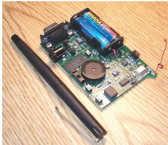
Figure 5. Prototype SpotON radio tag. These tags use radio signal attenuation to perform ad hoc lateration. Ad hoc clusters of tags cooperate to factor out measurement errors for all tag positions.
