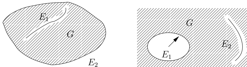
Figure 4: Ring domains
