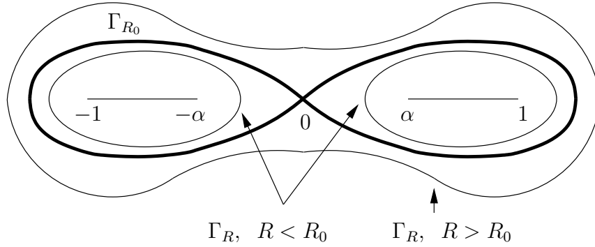
Figure 3: Level curves of g_{C \setminus E} for Example 4.2
