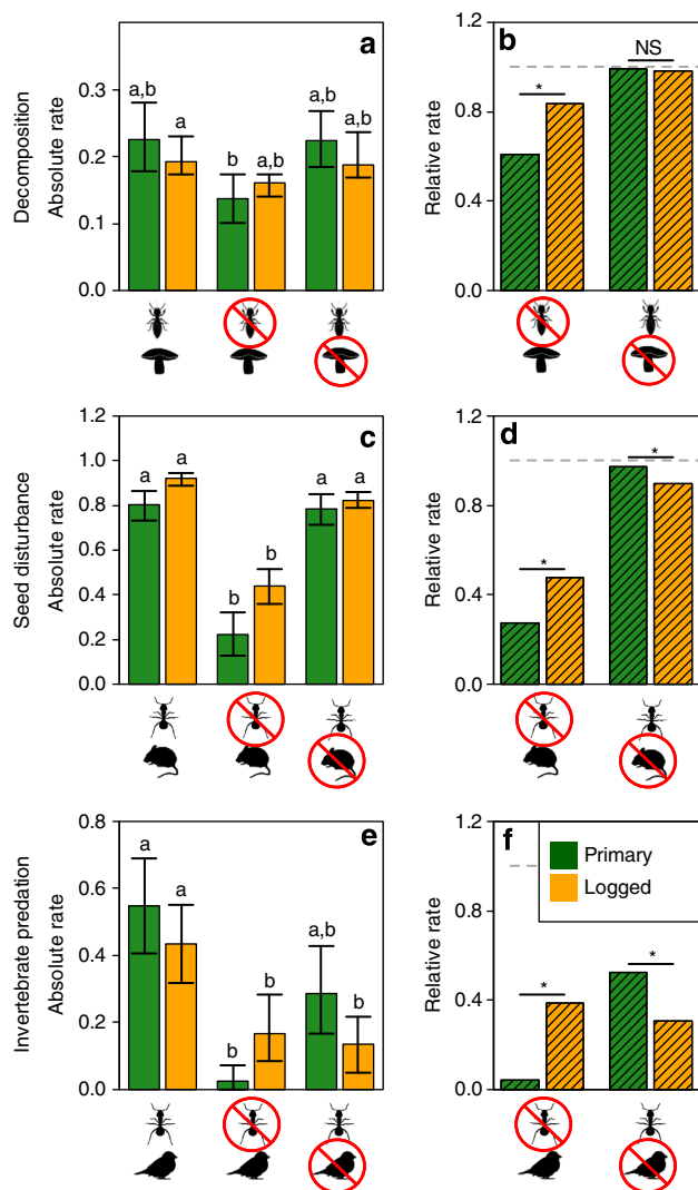
Figure 1 | Ecosystem process rates in primary (green) and logged (orange) forest in response to experimental removal of invertebrates, fungi or vertebrates. Ecosystem processes were quantified at three trophic levels represented by (a,b) leaf litter decomposition rate, (c,d) seed disturbance, defined as the combined removal and/or predation rate; and (e,f) invertebrate predation rate. Symbols indicate the taxa that contributed to the rates displayed. Absolute values (mean \pm 95% CI) of the ecosystem process rates are presented in the left-hand column and are measured as (a) the slope of a linear regression model relating log e -transformed litter mass (g) as a function of log e -transformed time (number of days), (c) the proportion of experimental seeds removed or predated per day, and (e) the proportion of experimental mealworm larvae predated per day. Letters indicate habitat × treatment categories that did not significantly differ from each other ( P < 0.05 ). There was a significant treatment × habitat interaction for all three ecosystem processes, demonstrating that the role of invertebrates was stronger in primary than logged forests. In the right-hand column (panels b,d,f), values represent the proportional change in ecosystem process rates relative to control sites (calculated from data presented in the left-hand column). Values <1 (dashed line) indicate functions whose rate is reduced following the exclusion of a taxon; smaller values indicate larger reductions in the rate and hence a stronger contribution of that taxon to delivering the ecosystem process. Posthoc significance tests were used to examine the treatment × habitat interaction effects. For example, in panel b, the asterisk indicates that the effect on decomposition of excluding invertebrates was significantly ( P < 0.05 ) larger in primary forest than in logged forest. NS indicates nonsignificant interactions.
