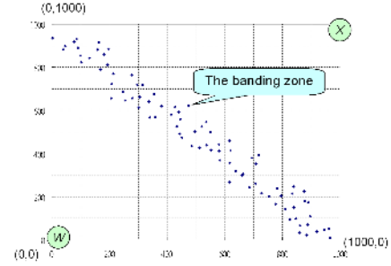
Fig. 8. An example for the distribution of nodes which satisfy w = x or w = x \pm 1 .
