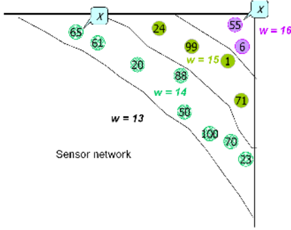
Fig. 6. A local flooding example for W_{\text{threshold}} = 14 .
