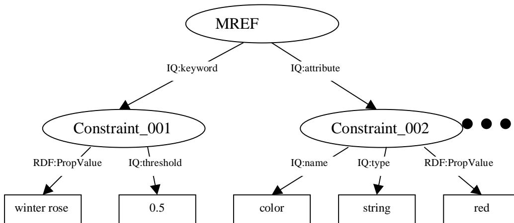
Figure 4: RDF Model for MREF
