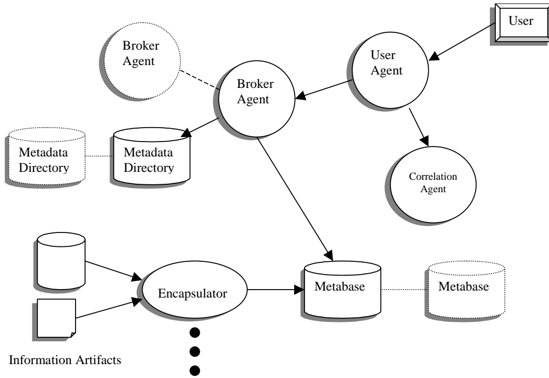
Figure 1: High Level InfoQuilt Architecture
