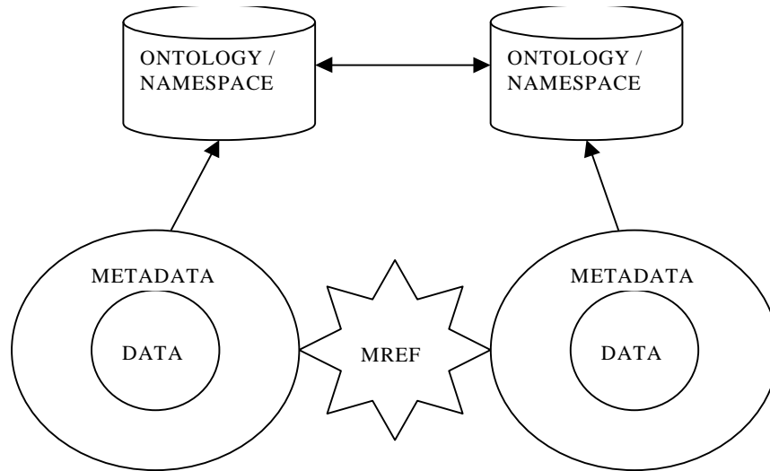
Figure 2: Abstraction Layers
