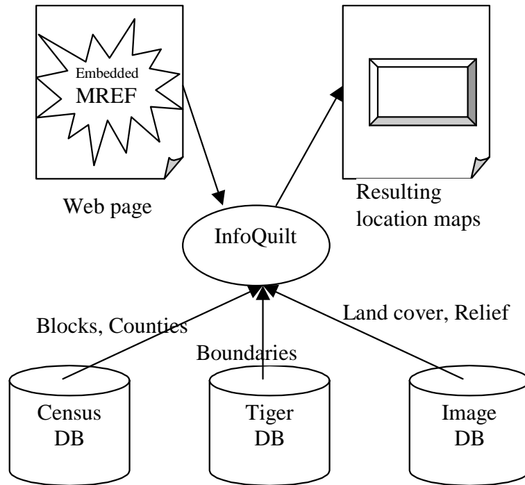
Figure 5: MREF correlation over heterogeneous sources
