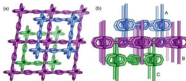
Fig. 1 View of the 2D \rightarrow 3D polythreading architecture from [111] (a) and [010] direction (b). Two dangling DMF pendants (simplified by sticks for clarity), from the adjacent layers above and below (A and C), thread each window of the central one (B).
