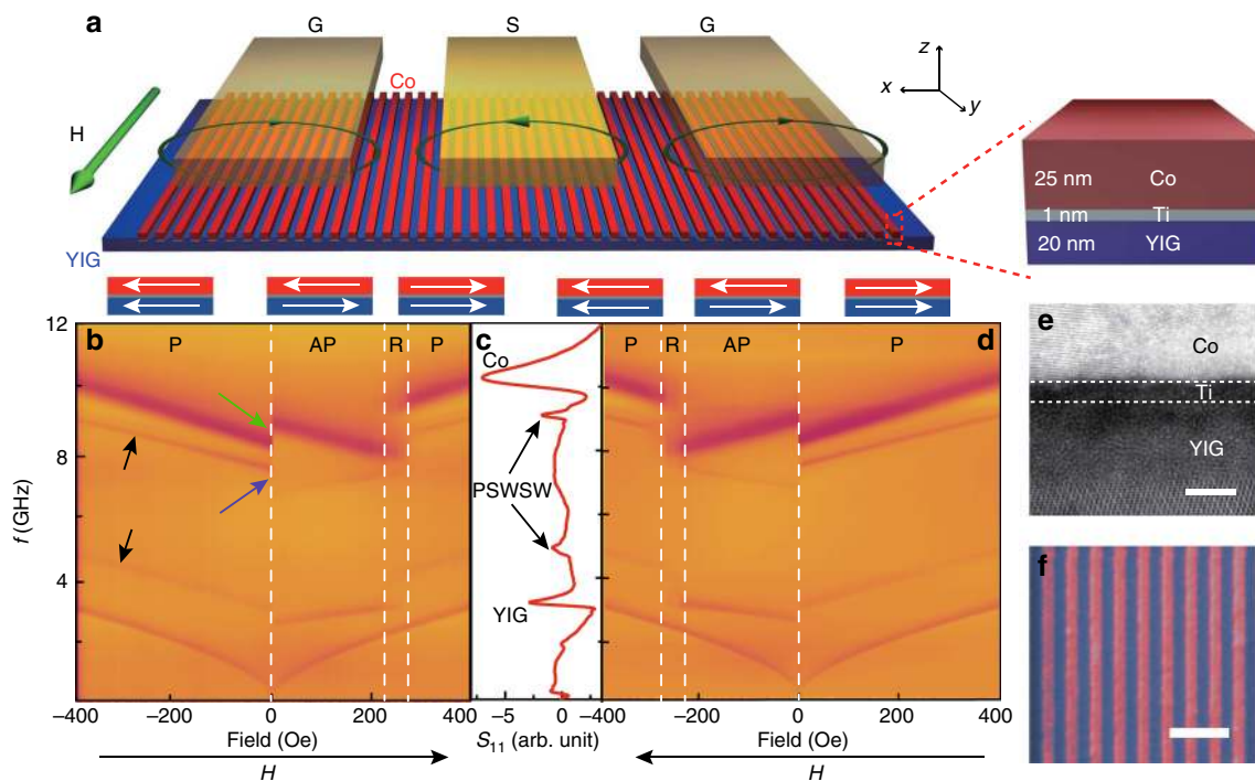
Fig. 1 Different magnetic states in a nanopatterned magnetic heterostructure. a Sketch of an YIG (20 nm)/Ti (1 nm)/Co (25 nm) heterostructure with a coplanar waveguide (CPW) prepared on the top. The applied field H is parallel to the Co nanowires (along the y axis). b Color-coded reflection spectra S_{11} measured on the device structure shown in a . The field is set to -3000 Oe to magnetize the Co nanowires and the YIG film to saturation first and then swept from -400 Oe to 400 Oe with a field step of 2.5 Oe. The spectra have several different regions corresponding to three different magnetic states: parallel state ( P ), antiparallel state ( AP ), and random state ( R ). c A line plot extracted from b at a field of 400 Oe. d Color-coded reflection spectra S_{11} with a reversed field sweeping direction, as indicated. The field is set to 3000 Oe first and then swept from 400 Oe to -400 Oe with a field step of -2.5 Oe. e TEM image of the YIG/Ti/Co heterostructure. The horizontal scale bar is 2 nm long. f SEM surface image of the heterostructure. The Co nanowires are color-coded in red and the YIG film beneath the wires are in blue. The scale bar is 500 nm long
