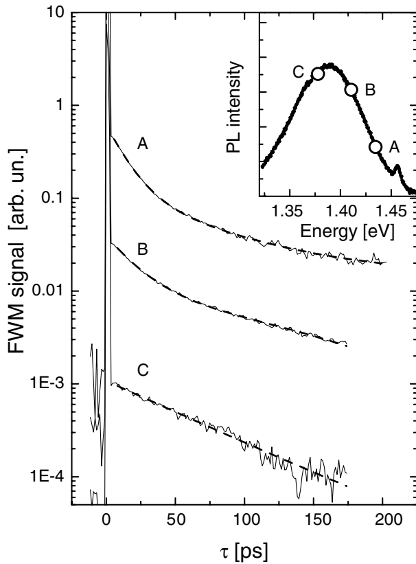
FIG. 1. Transient wave mixing. The data are taken for three different detunings of the laser ( A , B , and C ) as indicated in the inset, which also shows the sample luminescence spectrum. The small PL peak at around 1.45 eV is impurity-related emission from the sample substrate.
