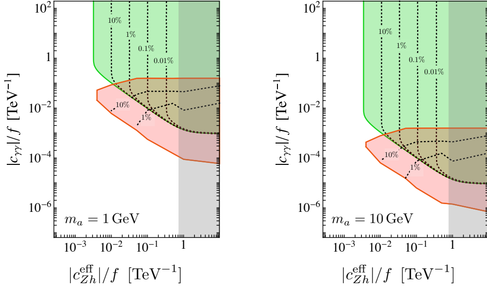
Fig. 67: Projected reach in searches for h \rightarrow Za \rightarrow \ell^+\ell^- + 2\gamma decays with ATLAS/CMS (green) and MATHUSLA (red) with \sqrt{s} = 14 TeV center-of-mass energy and 3000 \text{ fb}^{-1} integrated luminosity. The parameter region with the solid contours correspond to a branching ratio of \text{Br}(a \rightarrow \gamma\gamma) = 1 , and the contours showing the reach for smaller branching ratios are dashed. This estimate assumes the 200m \times 200m \times 20m benchmark geometry of Fig. 1.
