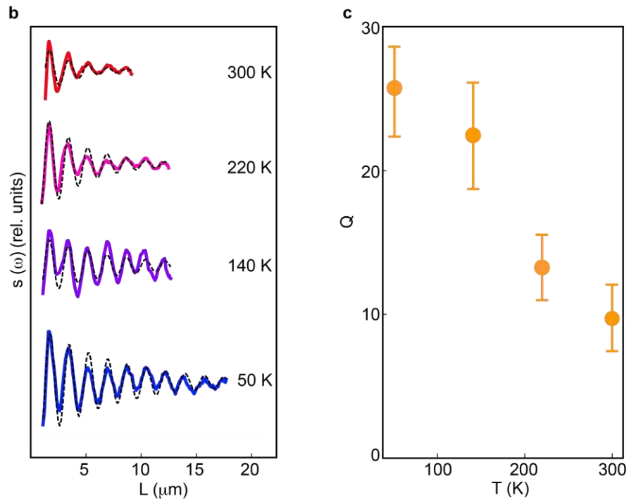
Figure 3. Temperature dependence of phonon polariton propagation in \alpha - \text{MoO}_3 crystals. a, Nano-IR images of the normalized near-field scattering amplitude s acquired at sequential sample temperatures from \alpha - \text{MoO}_3 crystals. A pair of gold disks beneath the \alpha - \text{MoO}_3 crystal function as antennas that emit polaritonic waves. b, Line profiles of phonon polariton fringes propagating from left to right, as a function of the distance L from the gold launcher. Dash-dotted lines represent the results of numerical simulations performed to identify the temperature dependence of the complex
