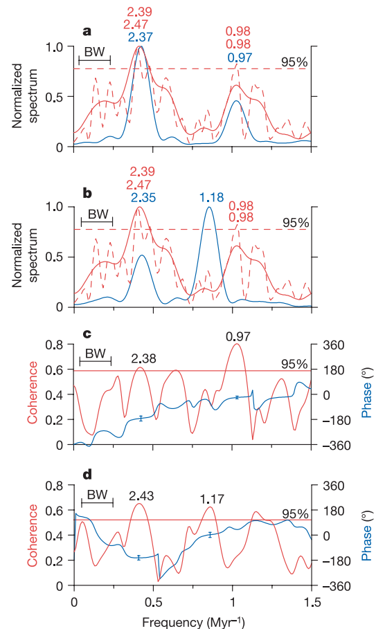
Figure 2 | Individual and cross spectra of turnover, eccentricity and obliquity. Methods used were Blackman–Tukey (solid lines), and CLEAN 30 (dashed lines). Numbers refer to significant periods (Myr). BW, bandwidth (for Blackman–Tukey). a , Red lines, per-taxon turnover. Blue line, eccentricity envelope ( \sim 100 kyr maxima). b , Red lines as in a . Blue line, obliquity envelope (41 kyr minima). c , Red line, coherence between per-taxon turnover and eccentricity maxima with 95% significance level for non-zero coherence. Blue line, phase difference; error bars (95% confidence level) are indicated for the relevant frequencies. d , Red line, coherence between per-taxon turnover and obliquity minima with 95% significance level for non-zero coherence. Blue line, phase difference; error bars (95% confidence level) are indicated for the relevant frequencies.
