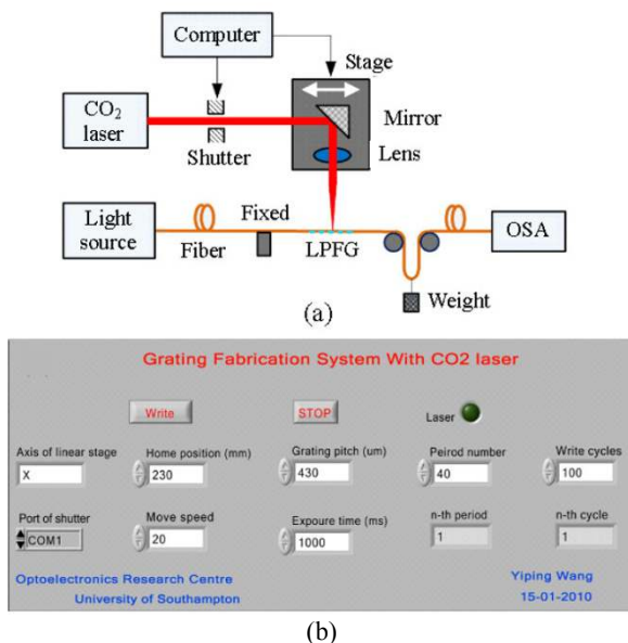
Fig. 3 LPFG fabrication system with a CO 2 laser: (a) the schematic diagram of an improved LPFG fabrication system employing a CO 2 laser and (b) the operation interface of the fabrication system.
