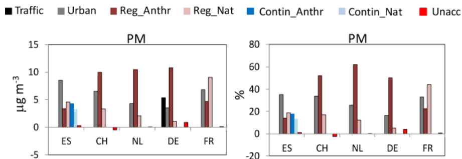
Figure 5. Lenschow's approach applied to the concentrations of PM 10 in the different countries (PM 2.5 in the Netherlands). Annual means are reported. ES: Spain; CH: Switzerland; NL: the Netherlands; DE: Germany; FR: France. In all countries with the exception of Spain, Reg_Anthr and Reg_Nat are the sum of the regional and continental increments.
