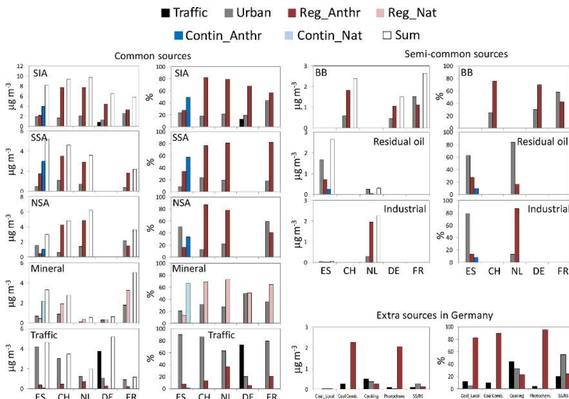
Figure 6. Lenschow's approach applied to the PM_{10} ( PM_{2.5} in the Netherlands) PMF source contributions. Annual means are reported. ES: Spain; CH: Switzerland; NL: the Netherlands; DE: Germany; FR: France. In all countries, with the exception of Spain, Reg_Anthr and Reg_Nat are the sum of the regional and continental increments. Lenschow's approach applied to the PM_{10} ( PM_{2.5} in the Netherlands) PMF source contributions. Annual means are reported. ES: Spain; CH: Switzerland; NL: the Netherlands; DE: Germany; FR: France. In all countries, with the exception of Spain, Reg_Anthr and Reg_Nat are the sum of the regional and continental increments.
