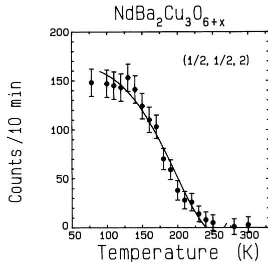
FIG. 3. Temperature dependence of the peak intensity of the (\frac{1}{2} \frac{1}{2} 2) antiferromagnetic peak, which is proportional to the square of the staggered magnetization. The rounding of the transition at T_N \sim 230 K is due to either critical fluctuations, or a distribution of T_N 's. The solid curve is a guide to the eye.
