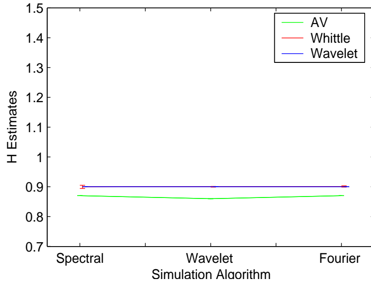
Figure 5: Summary of estimated Hurst parameters, for simulated FGN data. Curves are different estimation methods. Different simulation algorithms on the different axes. Error bars represent perceived likely variation in estimates. Shows very consistent estimation.
