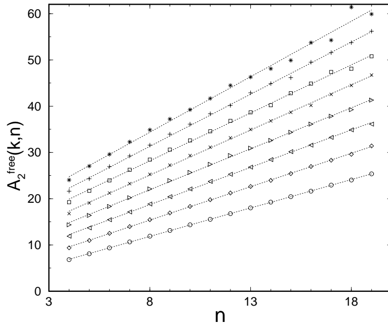
Figure 12. Free second-neighbour correlators A_2^{\text{free}}(k, n) (plotted for k even only) as a function of n for k = 4 (bottom line) to k = 18 (top line) for a foam without three-cells.
