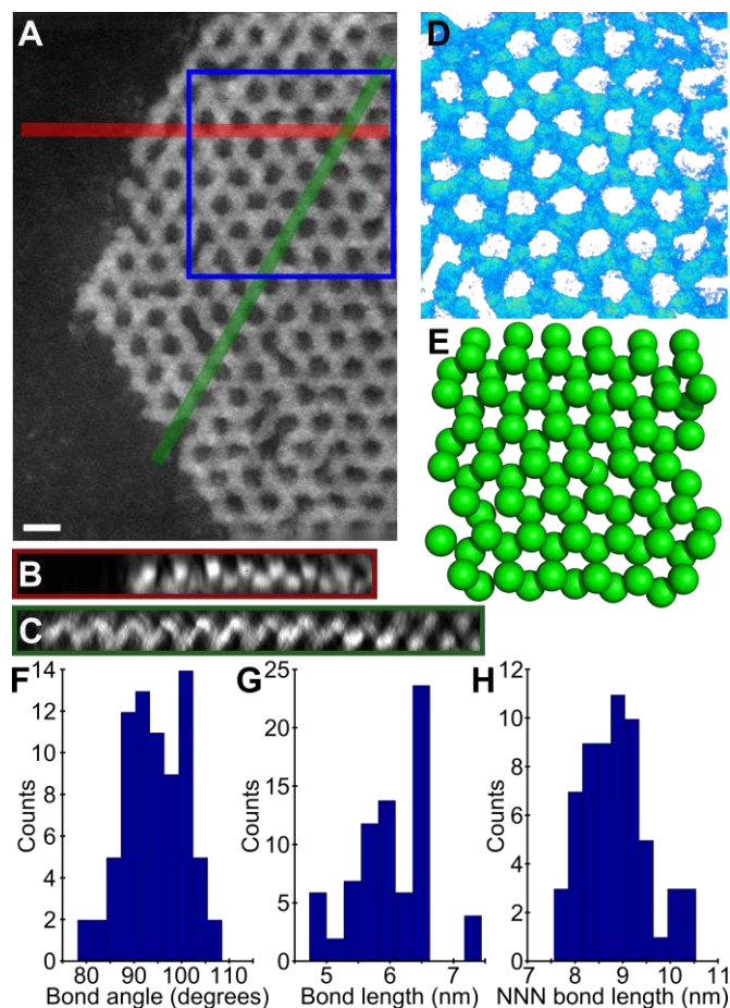
Fig. 3. HAADF-STEM tomography on a PbSe honeycomb structure. (A) Overview of the honeycomb structure obtained by averaging the tomographic reconstruction in the direction perpendicular to the substrate. Scale bar, 10 nm. (B,C) slices through the tomogram perpendicular to panel (A), along the (B) red, or (C) green line indicated in (A). (D) Iso-volume rendering of the tomographic reconstruction in the region indicated with the blue box in panel (A). (E) Equally sized spheres plotted on the coordinates obtained by automated particle detection in the region indicated in blue in panel (A). (F) Bond angles measured from the coordinates in (E), showing a bond angle of 95 \pm 5^\circ . (G) Bond lengths to nearest neighbors, showing a bond length of 6.0 \pm 0.5 nm. (H) Bond lengths to next-nearest neighbors, showing a NNN bond length of 8.9 \pm 0.6 nm.
