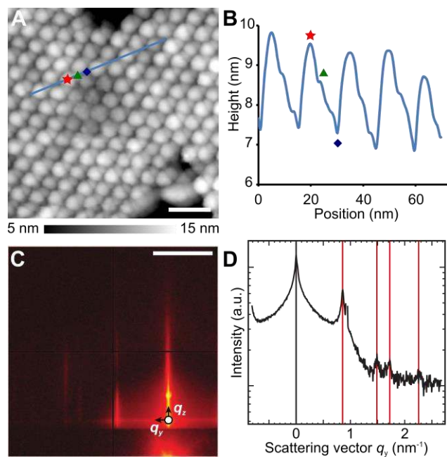
Fig. 2. STM and GISAXS measurements on the PbSe honeycomb structures. (A) Constant-current STM measurement showing high (red star) and low (green triangle) nanocrystals forming a honeycomb structure. Feedback settings 3.5 V and 20 pA; scale bar, 20 nm. (B) Height profile along the blue line indicated in (A) . The position of a high NC (star), low NC (triangle), and hollow site (diamond) are indicated. (C) GISAXS pattern of a honeycomb structure on top of a Si(100) substrate, under an angle of incidence of 0.7 degrees. Scale bar, 1 \text{ nm}^{-1} . (D) Line trace in the horizontal direction indicated in (C) , revealing the in-plane order. Red lines mark diffraction peaks with relative positions of 1:\sqrt{3}:2:\sqrt{7} , arising from the hexagonal order of the holes in the structure.
