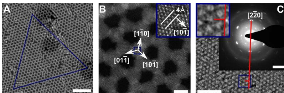
Fig. 4. Single crystalline CdSe honeycomb structures created by cation exchange. (A) HAADF-STEM image of the CdSe honeycomb structure. The honeycomb appears bright on a dark background. The equilateral triangle shows that the long range ordering of the structure is retained. Scale bar, 50 nm. (B) High-resolution HAADF-STEM image showing that the orientation of the Se anion lattice with respect to the superlattice geometry is preserved. Inset: zoom-in on the area indicated by the blue box. Scale bar, 5 nm. (C) An ED pattern showing that the high degree of crystallinity is preserved. TEM image in the background shows the area on which the ED pattern was recorded (the honeycomb appears dark on a bright background). Red line and inset show the orientation of the diffraction spots with respect to honeycomb structure, confirming that the \langle 110 \rangle axes are perpendicular to the NC bonds. Scale bar, 50 nm (TEM), 5 nm -1 (ED).
