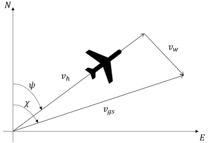
Fig. 3. Wind triangle.
