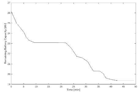
Fig. 18. Battery Discharged.
