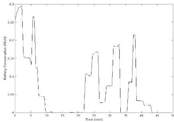
Fig. 17. Battery Consumption.
