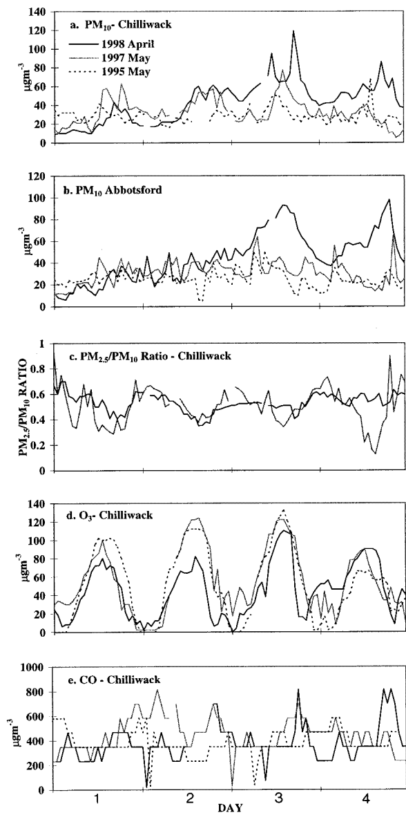
Figure 4. Four day times series of (a) PM_{10} at Chilliwack, (b) PM_{10} at Abbotsford, (c) PM_{2.5}/PM_{10} ratios, (d) O_3 , and (e) CO concentrations at Chilliwack for April 27–30, 1998, and meteorological analogs May 27–30, 1995 and May 12–15, 1997.
