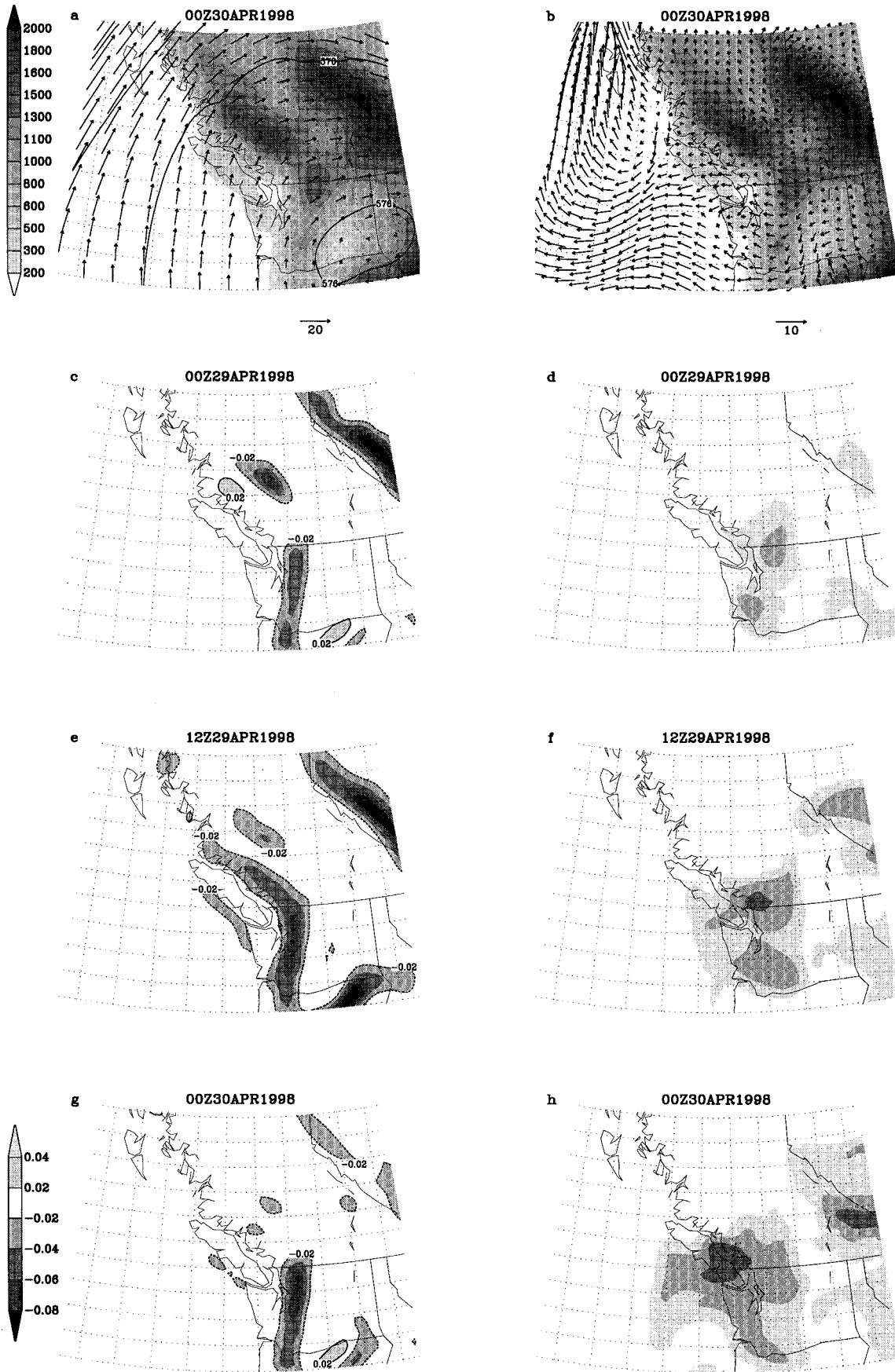
Figure 7. Numerical model simulation results from 0000 UTC, April 29, 1998 to 0000 UTC, April 30, 1998, showing (a) 500 hPa geopotential heights and wind vectors ( \text{m s}^{-1} ) overlaying topography (m), and (b) Surface (10 m) wind vectors and topography at 0000 UTC, 30 April. Below are couplets of panels showing (left) time sequence of surface layer vertical velocities ( \text{m s}^{-1} , subsidence is negative) and (right) surface tracer concentrations (dimensionless, highest concentrations are darkest).
