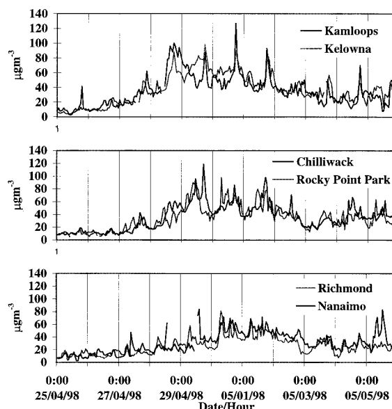
Figure 2. Time series of hourly PM_{10} concentrations for stations plotted east (top) to west (bottom) for the period 0000 Pacific standard time (PST), April 25, to 0000 PST, May 5, 1998 (dates are dd/mm/yy).
