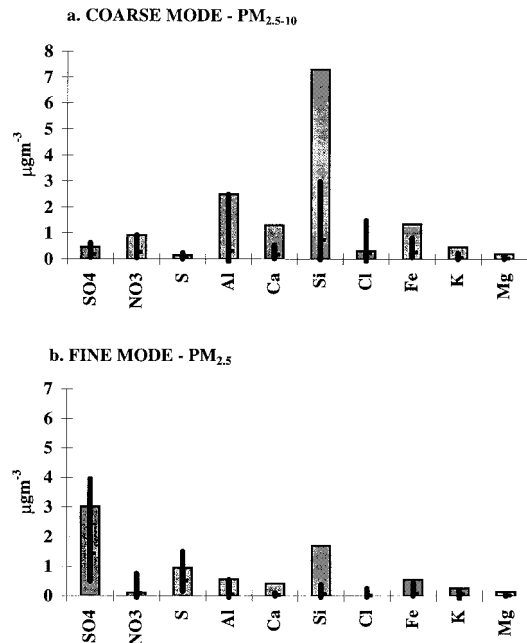
Figure 6. Concentrations for April 29, 1998 (solid bars) at Rocky Point Park, Vancouver, for selected ions and elements compared to historical (1996–1998) 99th percentiles (extent of top whisker), means (horizontal bar), and standard deviations (extent of bottom whisker) for (a) coarse mode particles ( PM_{2.5-10} ) and (b) fine mode particles ( PM_{2.5} ).
