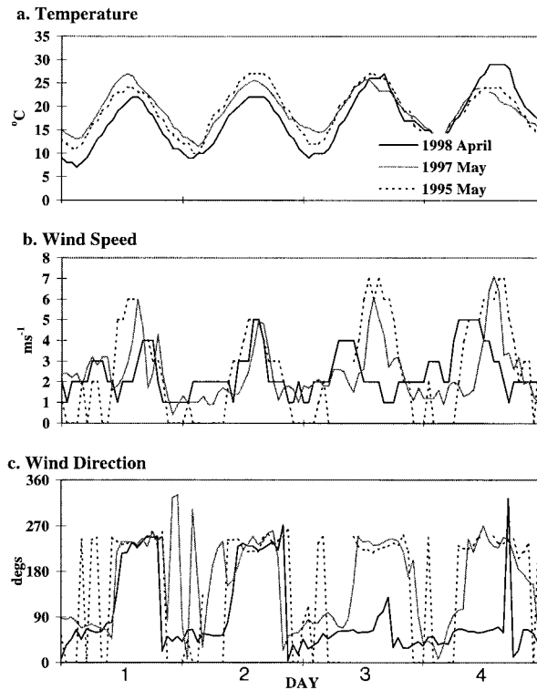
Figure 3. Four day times series of (a) temperature (b) wind speed, and (c) wind direction at Chilliwack for April 27–30, 1998, and meteorological analogs May 27–30, 1995 and May 12–15, 1997.
