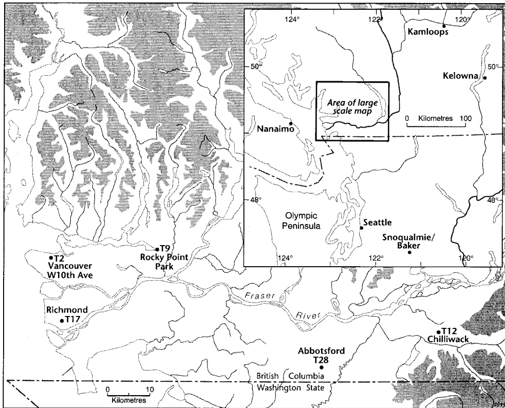
Figure 1. Map of the Lower Fraser Valley and wider region showing places mentioned in the text.
