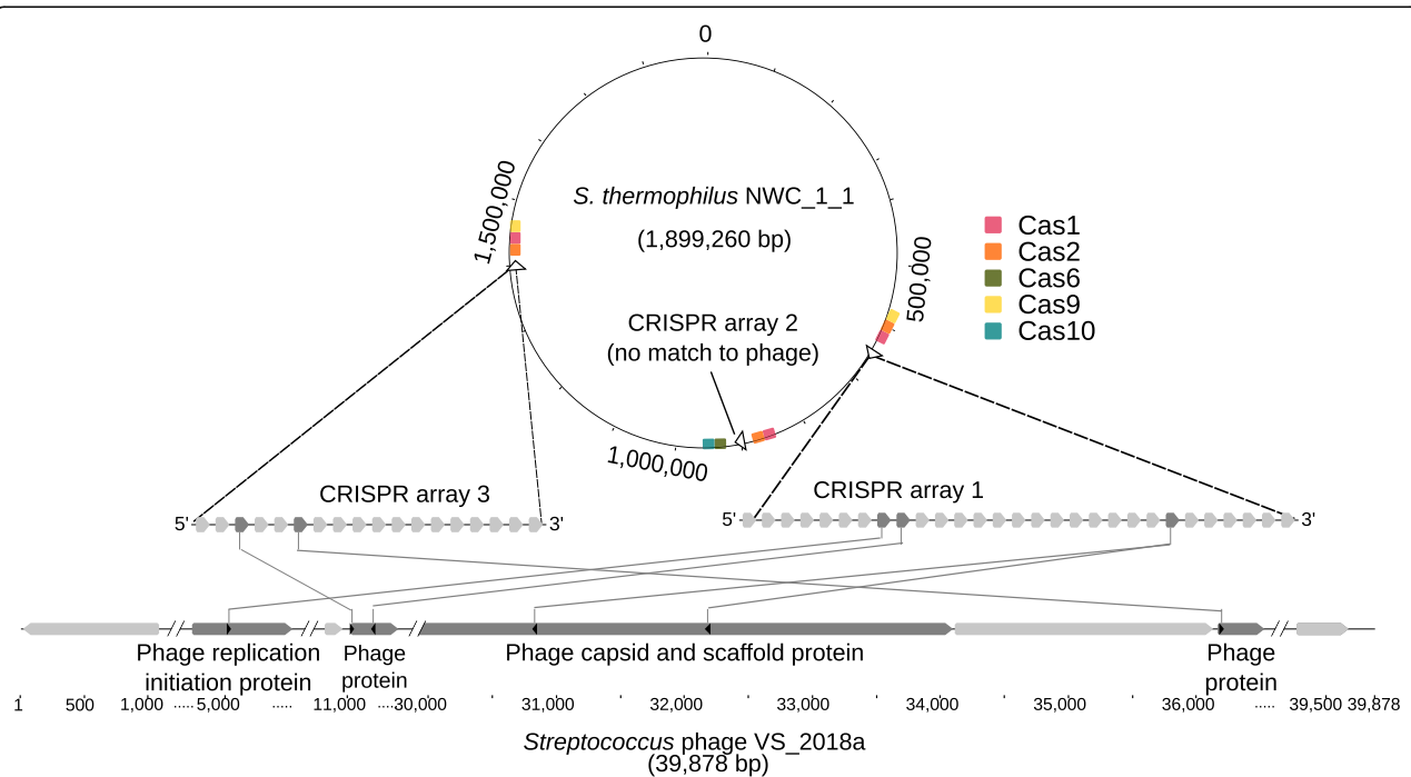
Fig. 6 CRISPR spacers in S. thermophilus strain NWC_1_1 and the S. thermophilus phage genome. Three CRISPR arrays (open arrows) and their flanking Cas genes are shown in the genome of strain S. thermophilus NWC_1_1 (top). CRISPR arrays 1 and 3 have matching spacers with the phage, as shown in the zoomed regions of the ~40 kb phage genome along with the annotation of selected phage protein-coding genes (bottom)
