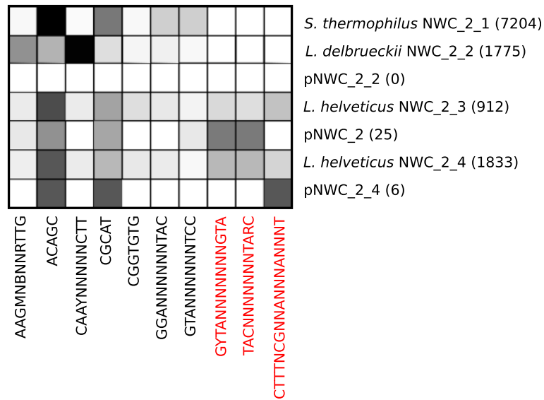
Fig. 5 DNA methylation motif analysis. The sequence and abundance of DNA methylation motifs were determined in all de novo assembled genomes of NWC_2 with the base modification module of the SMRTlink (v.5.1.0) toolkit and visualized. The heatmap illustrates the relative abundances of the motifs per assembly (increasing relative abundance from white to black). The numbers in the brackets represent the number of DNA methylation motifs detected in a given assembly. Motives specific to the L. helveticus strains and plasmids are highlighted in red
