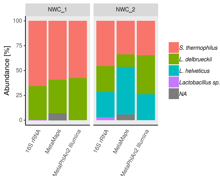
Fig. 3 Taxonomic profiling of NWC_1 and NWC_2. The relative abundances of predominant species in NWCs (see legend) are based on the 16S rRNA (v4) amplicon data, a MetaPhlan2 [36] analysis of the Illumina data, and a MetaMaps [37] analysis of the PacBio data for NWC_1 and NWC_2, respectively. NA = not assigned
