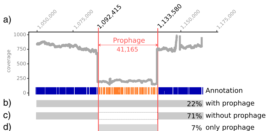
Fig. 7 Genome coverage of S. thermophilus NWC_2_1 around the prophage insertion site. a Genome coverage of S. thermophilus NWC_2_1 in the proximity of the prophage. Below the coverage plot, we highlight the prophage genome and its annotation as well as the percentage of reads that supported a respective variant. b The bacterial genome variant with the inserted prophage. c The dominant bacterial genome variant without the prophage. d The phage variant (here shown as linearized genome)
