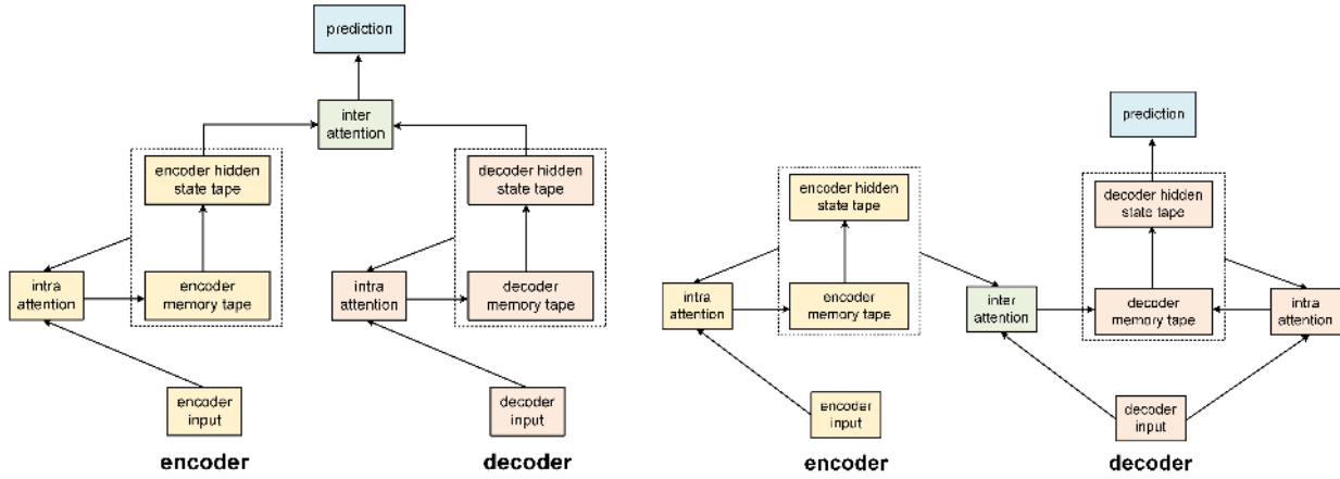
(a) Decoder with shallow attention fusion.
