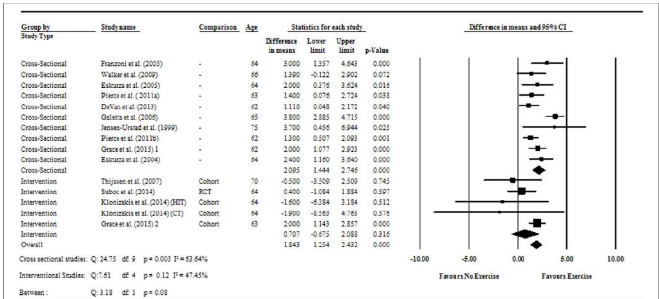
FIGURE 2 | Forest plot of the meta-analysis with mean differences of FMD percentage change between trained vs. sedentary healthy older adults (question 1), and FMD percentage change pre to post exercise intervention in previously sedentary healthy older adults (question 2). Outcomes of questions 1, 2, and the moderator analysis are also presented.
