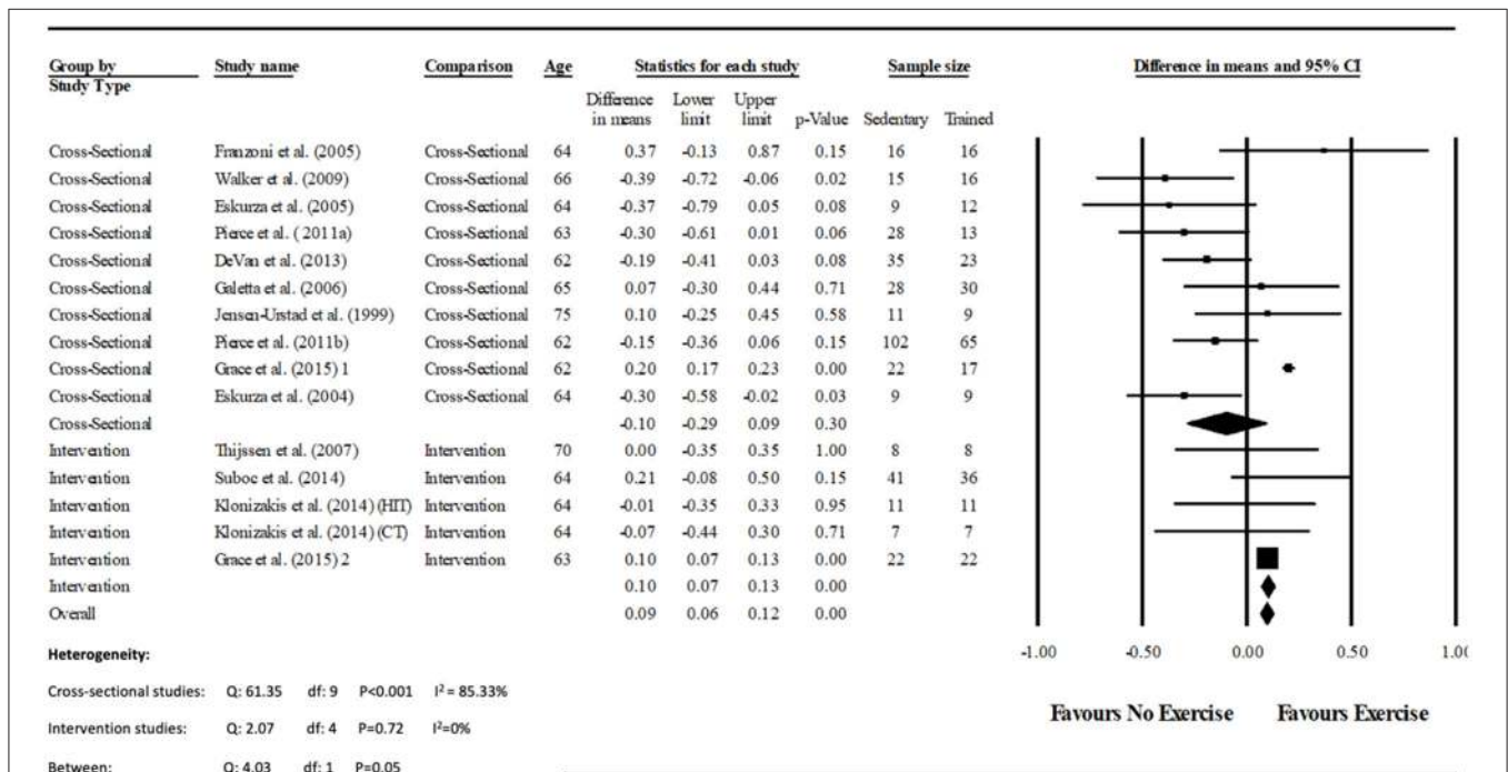
FIGURE 3 | Forest plot of the meta-analysis of brachial artery baseline diameter (mm) between trained vs. sedentary healthy older adults, and pre to post exercise intervention in previously sedentary healthy older adults. The heterogeneity and moderator analysis are also presented.
