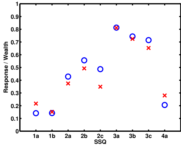
(b) SSQ Means in Model (blue circle) and Data (red x)
