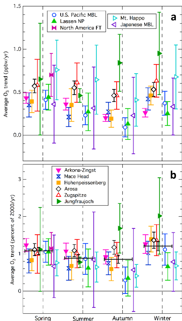
Fig. 7. Summary of average rate of increase in O 3 derived for the eleven northern mid-latitude data sets in each season. The order of the sites is the same as in Fig. 6. (a) Rates given as ppbv yr -1 derived from the slopes of linear regressions as described in the text. (b) Rates given as percentage of the year 2000 intercept defined as the ratio of the slope in (a) to the intercept in Fig. 6. The black plus symbols indicate the averages with confidence limits of these rates for all European and North American sites.
