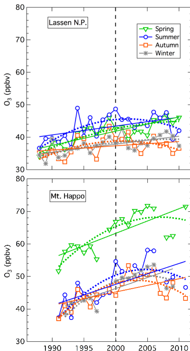
Fig. 4. Seasonal O_3 averages measured at high elevation ( \approx 1.9 km) sites in western North America at Lassen NP and in Japan at Mt. Happo. Lines indicate linear and quadratic regressions for the complete data sets in the same format as Fig. 2.
