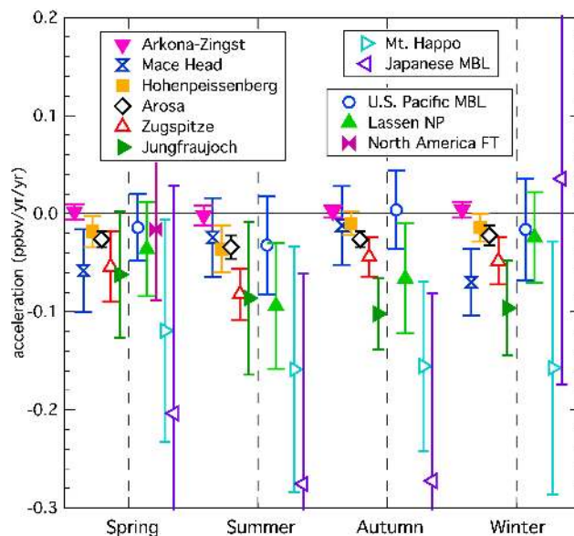
Fig. 8. Summary of the acceleration parameter derived from the quadratic regressions to the eleven northern mid-latitude data sets in each season. The acceleration, with units of ppbv yr -2 , is defined in Eq. (2) of the text, and represents the average rate of increase of the slope over the period of the data record.
