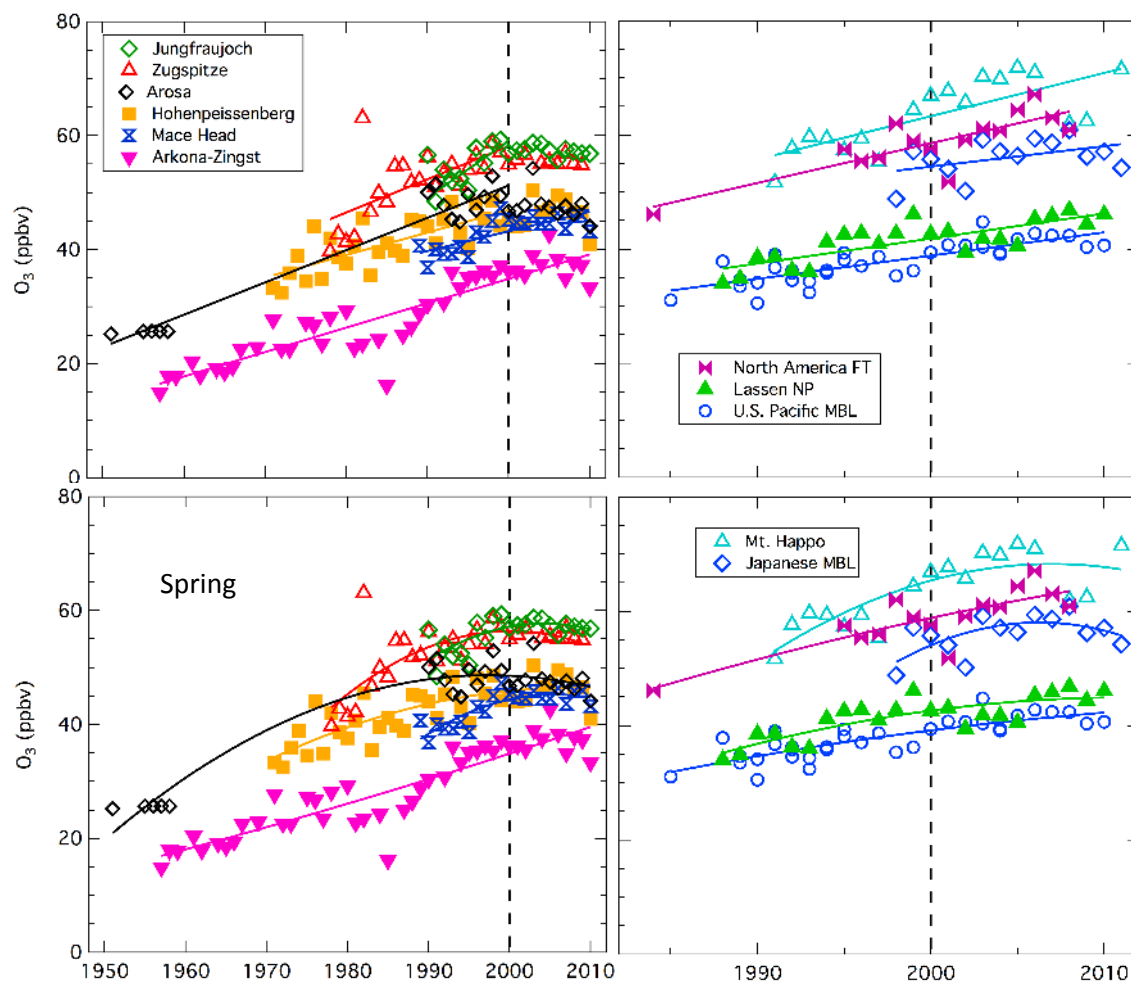
Fig. 5. Comparison of springtime trends in \text{O}_3 concentrations measured at all sites in Europe (left panels) and western North America and Japan (right panels). The lines (in color) indicate the linear (upper panels) and quadratic (lower panels) regressions to the data.
