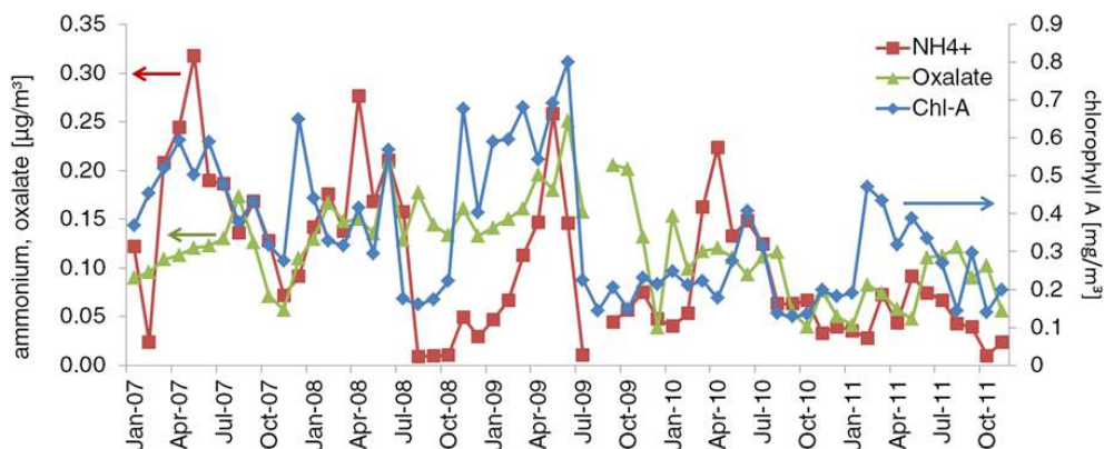
Figure 7. Monthly mean of chlorophyll a in the tropical NE Atlantic (selected area for averaging: lat (16.985, 24.895), lon (-24.87, -18.278)), oxalate and ammonium in PM_{10} aerosol samples collected at the CVAO.
