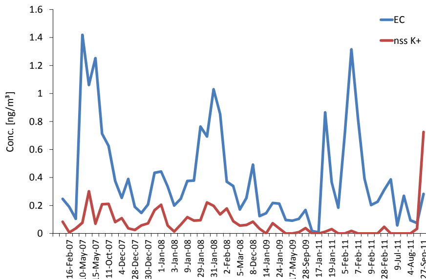
Figure 8. Time series of nss-potassium (nss-K + ) and elemental carbon (EC) measured during air mass inflow from Africa revealing similar temporal variations.
