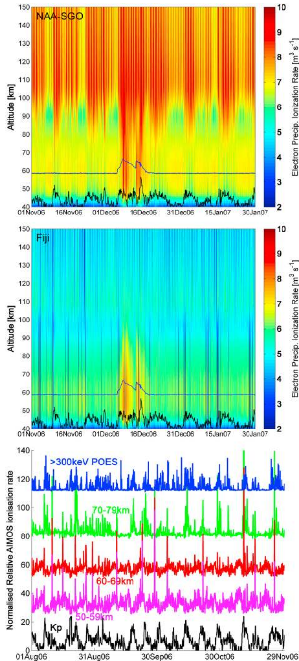
Figure 9. Ionization rates ostensibly due to electron precipitation reported by the AIMOS v1.2 model. (top) The rates for the NAA to SGO path. The black line shows the variability in the K_p geomagnetic index, and the blue line shows the GOES >10 MeV proton flux variation. (middle) The ionization rates above Fiji in the same format as the panel above. (bottom) The normalized variation in the AIMOS ionization rates for a range of mesospheric altitudes, with the >300 keV precipitating flux from POES EEP variation shown by the blue line and the K_p variation by the black line. Note that the Figure 9 (bottom) shows a different time range than Figure 9 (top and middle).
