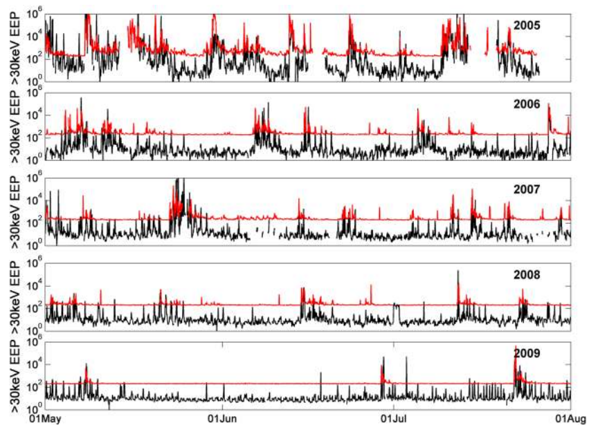
Figure 7. Comparison between the NAA-SGO-determined EEP flux magnitudes (black) and the MEPED/POES >30 keV electron fluxes (red) during the summer months over 5 years. In all cases, the fluxes are shown with units of \text{cm}^{-2} \text{s}^{-1} \text{sr}^{-1} . The change in activity level between solar minimum ( \sim 2009 ) and near solar maximum (2005) can easily be recognized.
