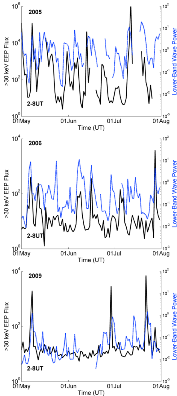
Figure 8. The variation in the NAA-SGO-determined EEP flux magnitudes (black line) contrasted with the varying lower band chorus wave intensity (blue line) observed from the DEMETER satellite. In both cases, the median over 02:00–08:00 UT is taken for each year.
