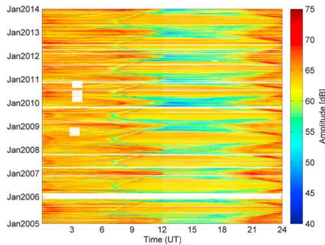
Figure 2. Slightly more than 9 years of 1 min resolution median amplitudes of the transmissions from NAA received at Sodankyla (SGO), Finland. The colors represent the amplitude of the received signal in decibel relative to an arbitrary reference level. The white regions correspond to either missing or removed (unreliable) data.
