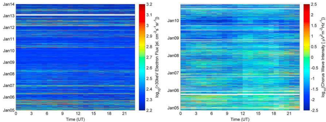
Figure 3. (left) Variation in the median hourly POES 0^\circ >30 keV electron flux averaged across L = 3 - 7 . The 0^\circ electron telescope measures electrons deep inside the BLC. (right) Hourly median DEMETER observations of lower band chorus mode wave intensity averaged across L = 3 - 7 , with no MLT restriction.
