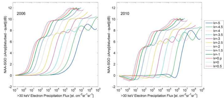
Figure 6. Daytime LWPC modeling of the amplitude changes due to EEP fluxes for the path NAA-SGO for (left) 2006 and (right) 2010. The energy spectra of the precipitating electrons are specified using a power law which is varied through the k parameter. The modeling used the updated Wait ionosphere parameters for each year, shown in Figure 5.
