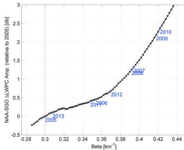
Figure 5. Change of the Wait ionosphere \beta parameter used in the LWPC modeling determined from the observed QDC noontime amplitude changes across the solar cycle.
