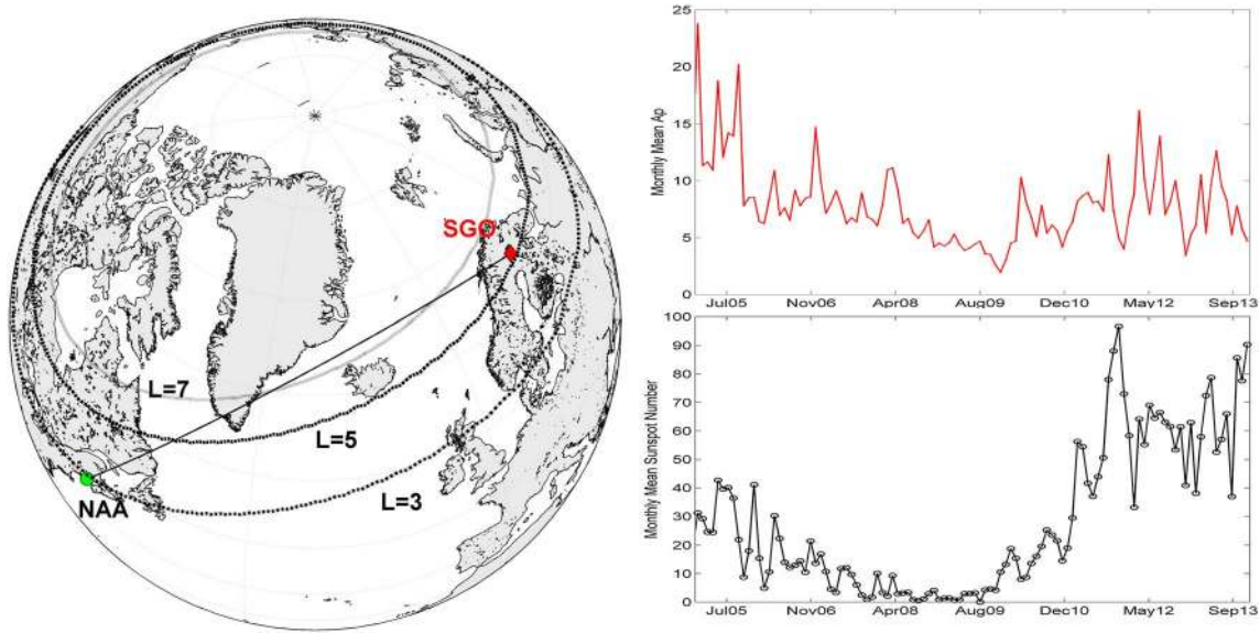
Figure 1. (left) Map of the subionospheric VLF propagation path from the NAA transmitter to the SGO receiver. The contours of constant L shell are shown indicating the atmospheric footprints of L = 3, 5, and 7 . (upper right) Monthly average A_p value for the period of November 2004 to December 2013. (lower right) Monthly average sunspot number over the same time period.
