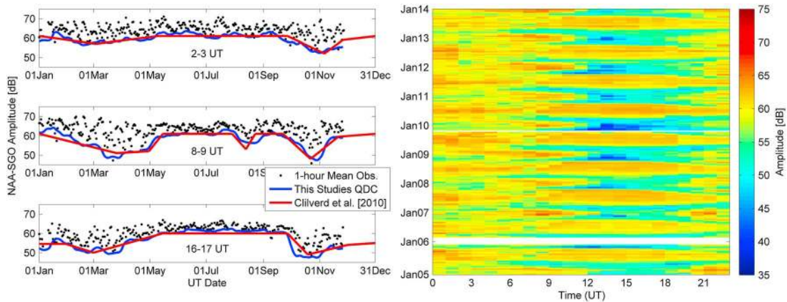
Figure 4. (left) Examples of QDCs generated in this study (blue) to represent the 2005 amplitude observations at 02:00–03:00, 08:00–09:00, and 16:00–17:00 UT. The QDCs for the same time spans presented in Clilverd et al. [2010] are shown in red for comparison. The new method follows the lower edge of the amplitudes more closely but is similar to that put forward in the earlier study. Note the large data gap in December 2005, which is also seen in Figure 2. (right) The QDC generated across our entire ~9 year time period.
