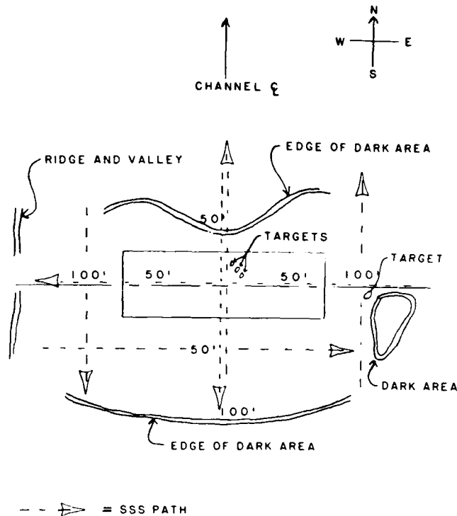
Figure 18. Completed sand cap coverage
