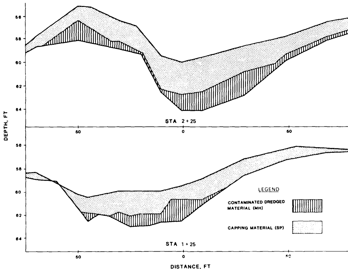
Figure 5. Typical composite profiles through completed disposal mound
