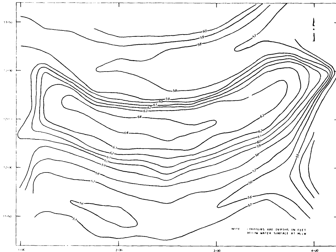
Figure 2. Bathymetry at disposal site
