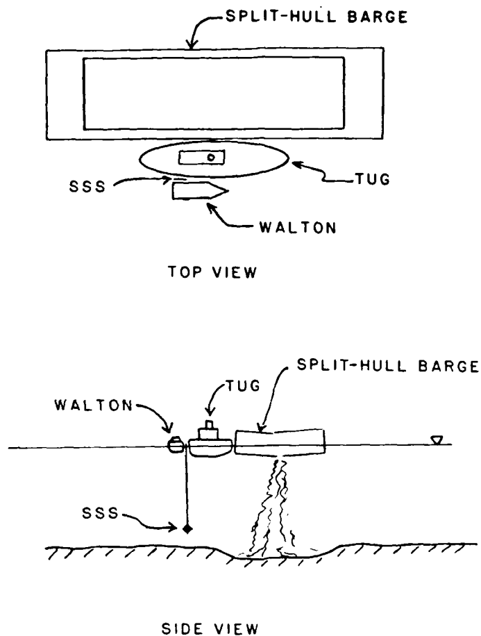
Figure 14. SSS positioning during dredged material disposal
