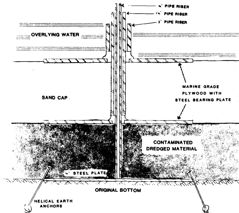
Figure 12. Schematic of tiered settlement plates
