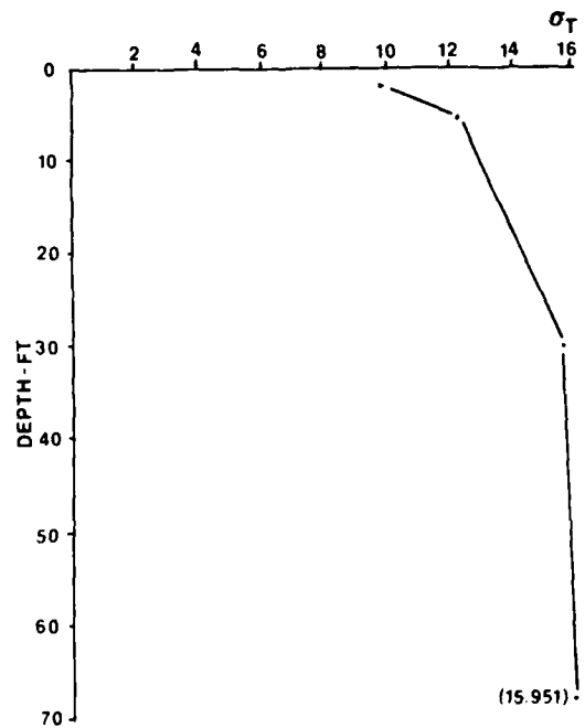
Figure 4. Physical parameters measured at disposal site
