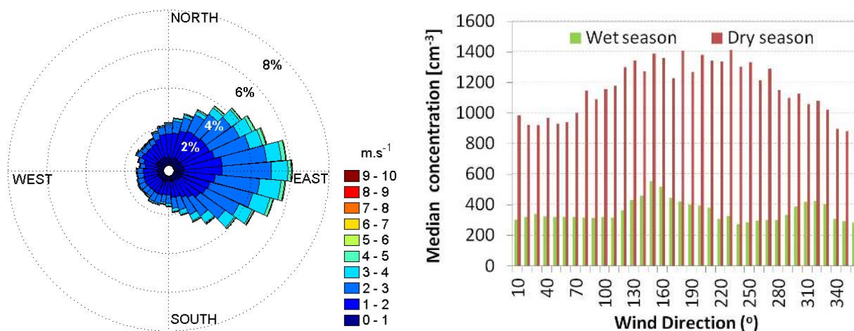
Fig. 3. (a) Wind rose plots for the period between January 2008 and June 2011. (b) Median aerosol particle number concentration as a function of wind direction for the wet season (January–June) and for the dry season (July–December). The Manaus city is located 60 km away in the southeast direction.
