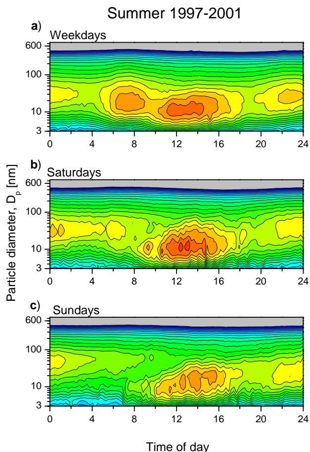
Fig. 3. Summer diurnal variation in the number size distribution averaged over (a) weekdays, (b) Saturdays, and (c) Sundays (June–August; 1997–2001). The colors represent the number concentration as dN/d\log D_p with grey as the lower limit corresponding to <200\text{ cm}^{-3} and red as the maximum corresponding to 45\,000\text{ cm}^{-3} .
