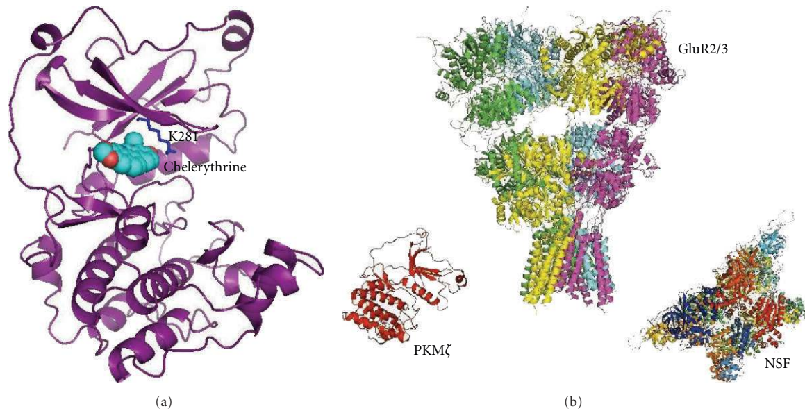
FIGURE 3: 3D models of proteins involved in the long-term memory maintenance: (a) human PKM \zeta homology model based on PKC iota [1ZRZ.pdb]. The chelerythrine (sphere-filled model with the oxygen atoms shown as red spheres and carbon atoms as cyan) binding site was identified within the ATP-binding pocket of the PKM \zeta (ribbons). Docking was performed using AutoDock software [117] and protein was visualized using PyMol. The inhibitor binding site is located in the vicinity of the Lys281 residue. K281W mutation renders PKM \zeta inactive and causes permanent erasure of the long-term memory [118]. (b) The N-ethylmaleimide-sensitive factor (NSF) consists out of two hexameric Walker-type D1 and D2 domains (N-terminal NSF domain not shown). Its ATPase-catalytic activity is needed to release GluR2 subunit from endosomes and GluR2/3 assembly at the postsynaptic membrane. Crystallographic structure for the last 68 amino acids of the GluR2 C-terminal, including the NSF and AP2 binding sites, is not available.
