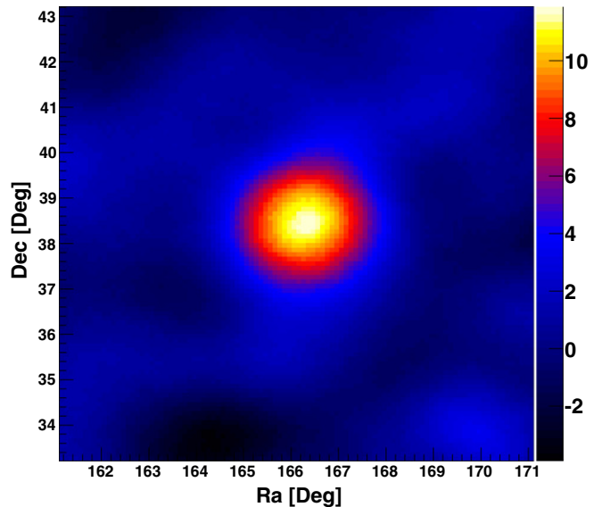
Figure 1. Distribution of statistical significance around Mrk 421. (A color version of this figure is available in the online journal.)
