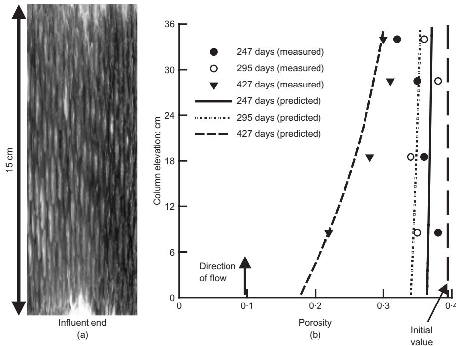
Fig. 9. Results from a column test using 6 mm glass beads: (a) glass beads at the end of a column test, showing greatest clogging at the bottom (influent end) and reduced clogging moving up the column; (b) observed and calculated variation in porosity with position at three times (data from VanGulck, 2003)
