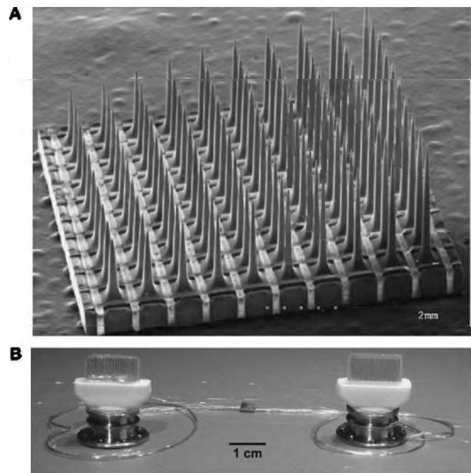
Fig. 1. Implanted device. (a) Scanning electron micrograph of the USEA). (b) Picture of the array, the lead wires and the connector system. Each connector is wired to 36 electrodes and two reference electrodes. The titanium pedestal of the connector itself is used as ground.
