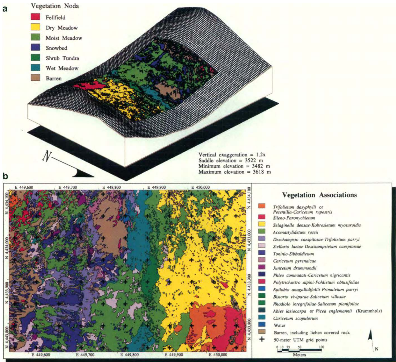
Figure 8. Vegetation, terrain, and snow depth on the Niwot Ridge Saddle grid. a. Vegetation nodas (May and Webber 1982) draped over a 3-D view of the Saddle. b. Vegetation associations mapped according to the classification of Komárková (1979). c. The snow map is interpolated from average May snow depths at the 88 grid points in 1982, 1983, and 1984. d and e. Slope and aspect maps derived from the digital terrain model. The bar graphs with each map portray the percentage of each map covered by the classes shown along the x-axes. Each bar is divided into sections representing the percentage of the class covered by the vegetation associations in b. The bottom cell of each bar represents the lumped total of vegetation types with area percentages too small to be shown as separate sections.
