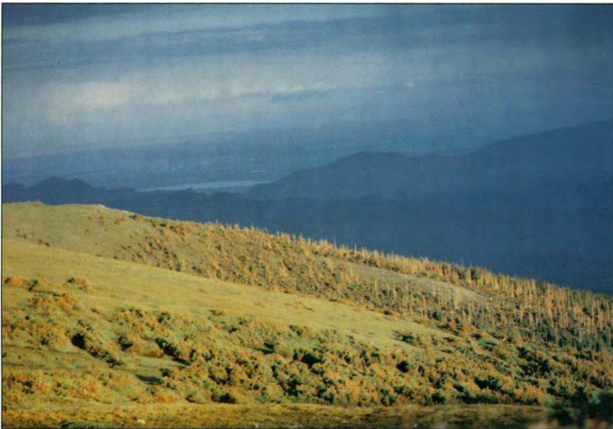
Figure 5. Treeline on Niwot Ridge. At the regional scale, HGIS focuses on phenomena associated with large-scale climate shifts, such as the position of the treeline and greenness of the tundra, which can be detected by means of remotely sensed data. Photo by J. C. Halfpenny.
