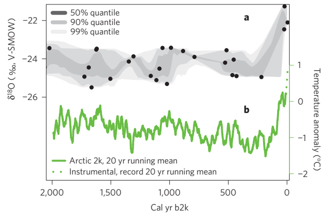
Figure 3 | Arctic temperature trends during the past two millennia.
