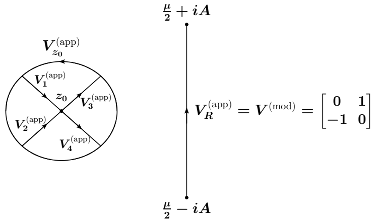
FIGURE 2.7. The RHP P^{(app)} for the plane-wave region. The circle r_{z_0}^{\epsilon} is enlarged to show detail.
