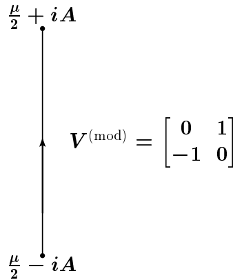
FIGURE 2.6. The RHP P^{(\text{mod})} for the plane-wave region.
