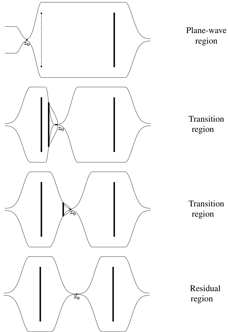
FIGURE 1.6. The final transformed RHP for decreasing values of \xi . The jump on the thin contours decay in time; the jump on the thick contours contribute to the leading-order solution. The dashed line in the first picture is not part of the RHP but indicates the \lambda_L cut.
