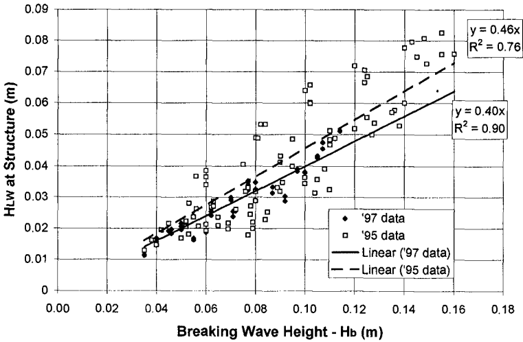
Figure 8 - Long Wave Height at the Structure and Breaking Wave Height
