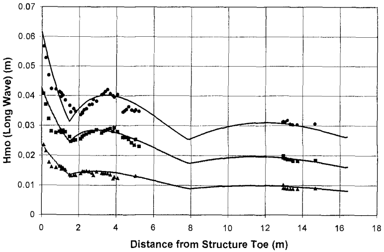
Figure 5 - Long Wave Height Profile
