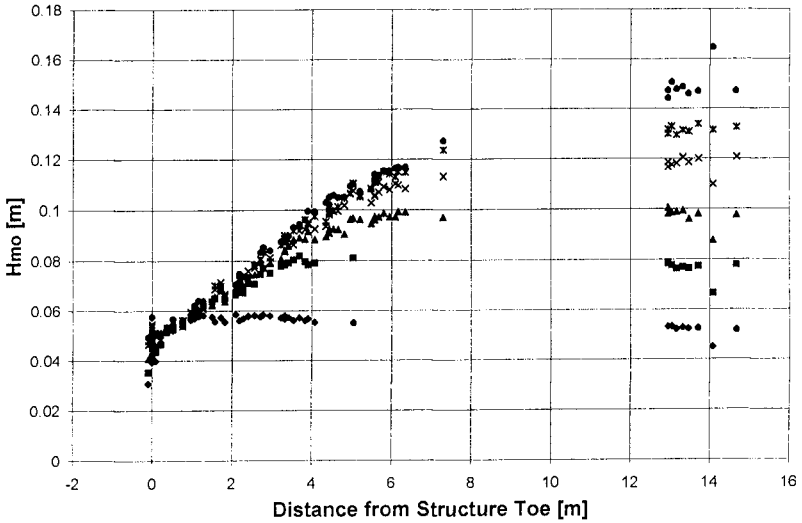
Figure 2 - Wave Height Profile
