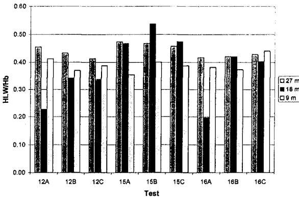
Figure 15 –Length of Wave Guides
