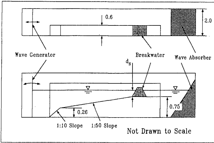
Figure 1 - Experimental Setup
