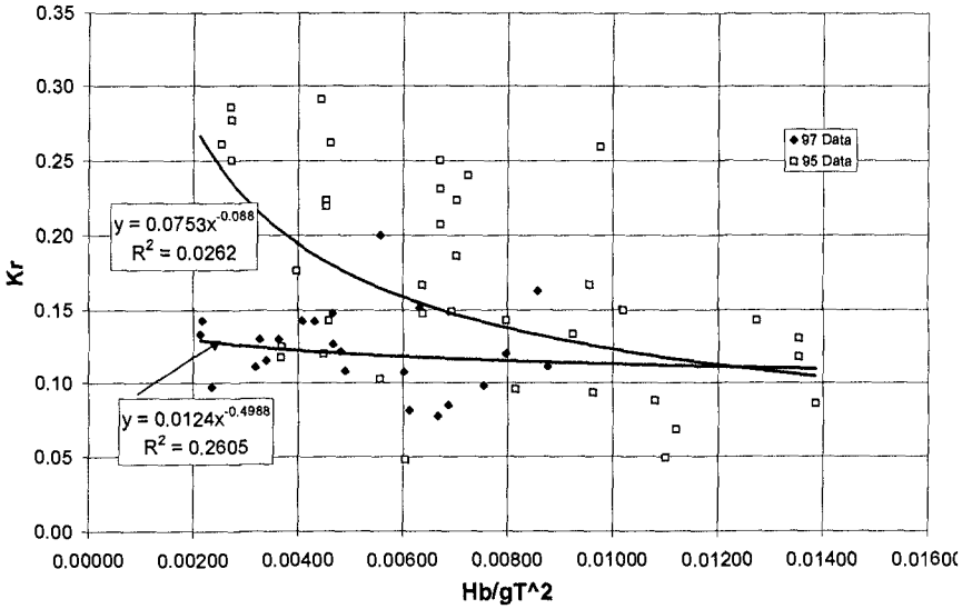
Figure 12 - Long Wave Reflection Coefficient
