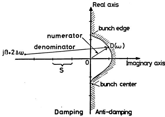
Fig. 3. The curve D(\omega) follows the real axis except for values of \omega within the band of incoherent synchrotron frequencies \omega_i .
