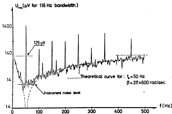
Fig. 4. Voltage at the input to the VCO and theoretical curve for no spread ( S = 0 ). Measured curve averaged 16 times.
