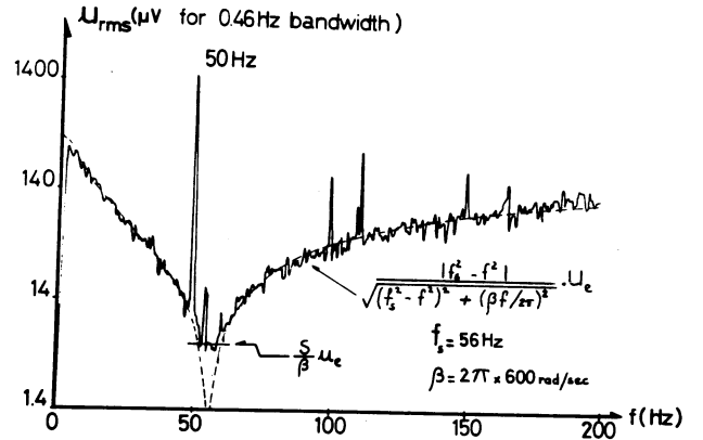
Fig. 5. Measured voltage with white noise added, and theoretical curve.
