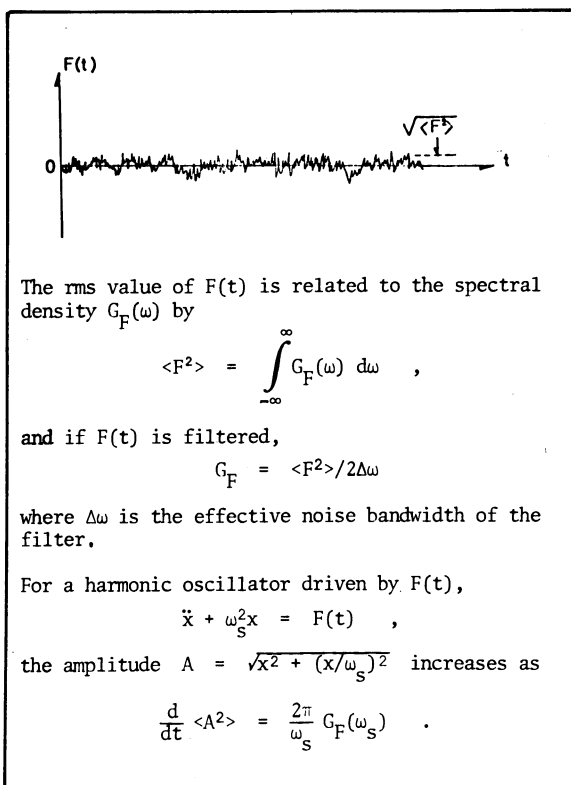
Fig. 1. Noise definitions. 1
