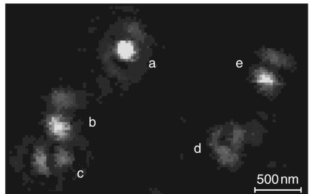
FIG. 4. Fluorescence rate images [R(x, y)] of arbitrarily oriented molecules excited with a focused radially polarized beam. The dipole moment of molecule a is nearly longitudinal (cf. Fig. 2D), whereas the dipole moments of molecules c and d are transverse. Molecules b and e have an orientation of \theta \approx 60^\circ (cf. Fig. 2C).
