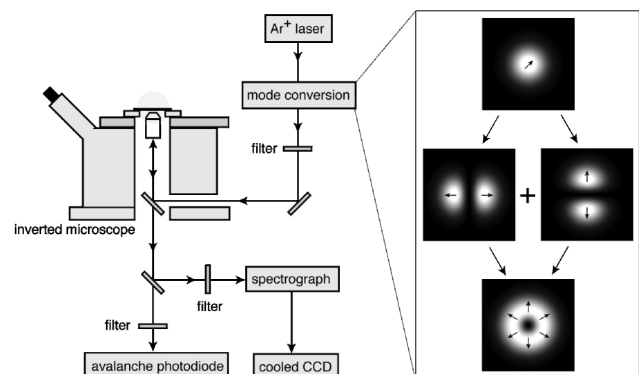
FIG. 1. Experimental setup: The fundamental laser mode of an Ar + laser ( \lambda = 488 nm) is converted into a radially polarized mode and focused on a dielectric sample consisting of a PMMA layer with embedded dye molecules. The strength of the longitudinal field at the laser focus is determined by scanning individual molecules with fixed absorption dipole orientation through the laser focus and monitoring the fluorescence emission rate.
