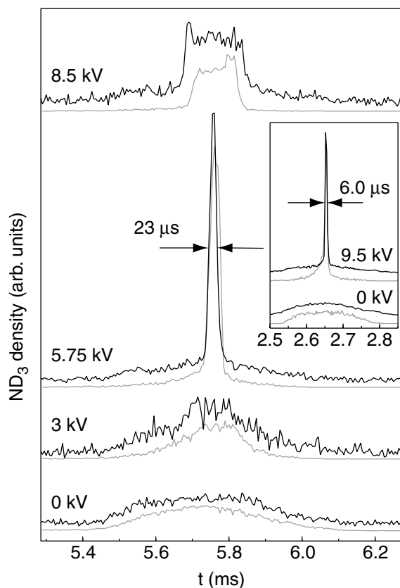
FIG. 3. Density of ammonia molecules 33 cm behind the buncher as a function of time (at t = 0 ms the synchronous molecule is at the exit of the decelerator) for different voltages on the buncher, using two bunching stages. In the inset similar measurements recorded at a 4.5 cm distance behind the buncher, using three bunching stages, are shown. The results of trajectory calculations through the entire setup are shown underneath the experimental data.
