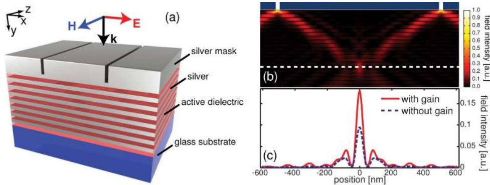
Fig. 8. (a) Schematic of the hypergrating structure. (b) Field intensity map plotted in the x - y plane at a wavelength of 716\text{ nm} with gain. (c) Field intensity plotted at a distance 345\text{ nm} into the HMM slab with gain (solid line) and without gain (dashed line). The dashed line in (b) indicates the position of the cross section of (c).
