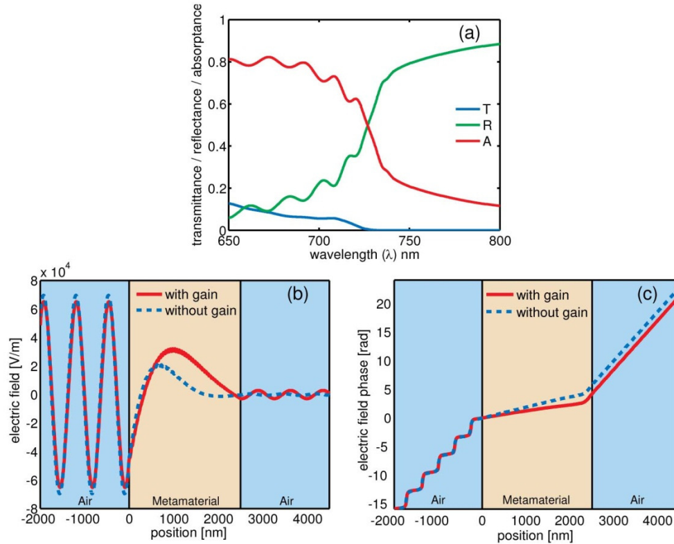
Fig. 10. (a) Transmittance, reflectance, and absorptance spectra calculated by SHA for a 100-layer silver-gain HMM with a silver-layer thickness of 5 nm and a gain-layer thickness of 45 nm. (b) Electric field and (c) the phase of the electric field plotted along the propagation direction at a wavelength of 729 nm with gain (solid line) and without gain (dashed line).
