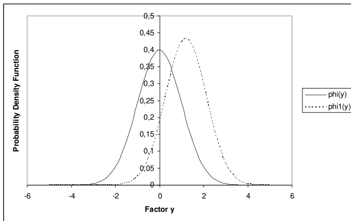
Figure 4. Density functions \phi and \phi_1
