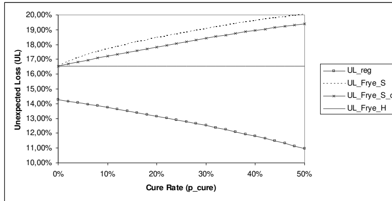
Figure 8. Regulatory and Frye model based 99,9% unexpected loss estimations depending on p_{cure} (with p_H = 2.5\% , \mu = 70\% , \sigma = 15\% , \rho = \rho_1 = 15\% , \rho_2 = 8\% )
