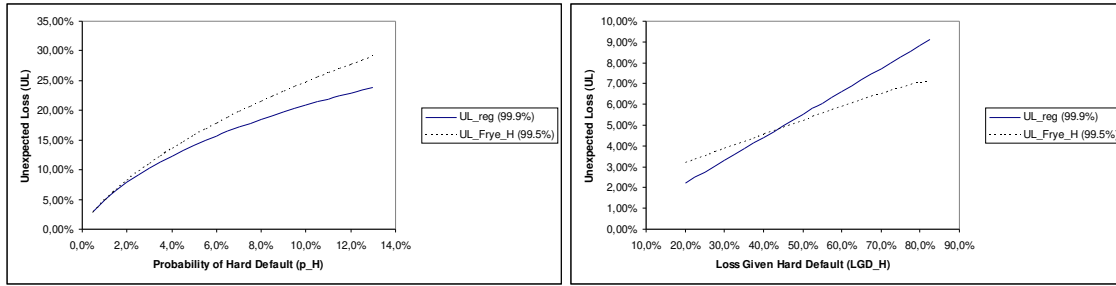
Figure 9. Sensitivity of the 99.9% regulatory and 99.5% Frye model unexpected loss on p_H and \mu (with, \sigma = 22\% , \rho = \rho_1 = 15\% , \rho_2 = 13\% , \mu = 45\% in the first graph, and p_H = 1\% in the second)
