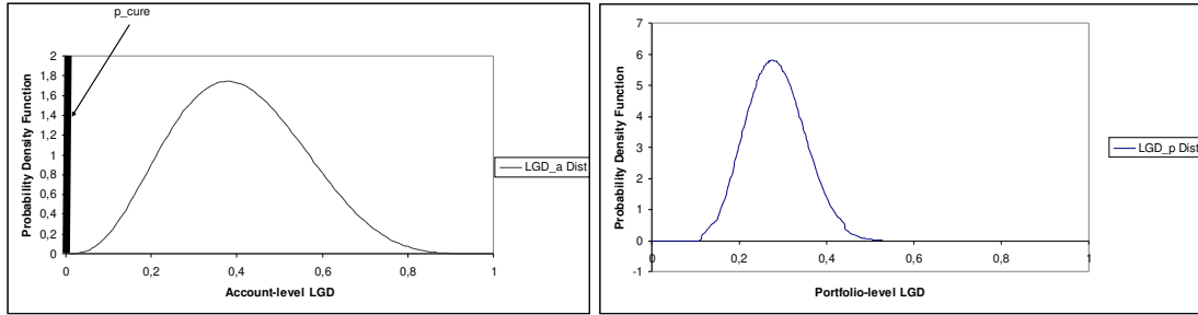
Figure 6. Account and transformed portfolio loss given default distribution ( p_{cure} = 0.3 , \mu = 0.4 , \sigma = 0.15 , \rho = 0.1 ).
