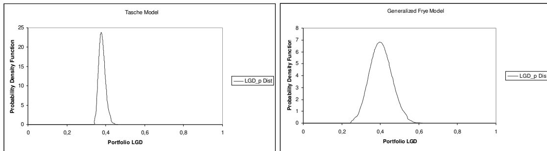
Figure 2. Portfolio loss distribution in the Tasche and generalized Frye model ( \mu = 0.4 , \sigma = 0.15 , \rho = 0.15 , p_H = 0.01 )
