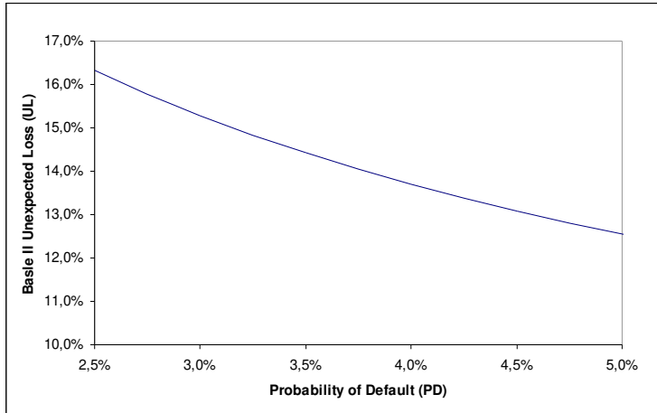
Figure 1. Unexpected loss according to the Basie II formula if EL=PD \cdot LGD=2\% is fixed and PD varies from 2.5% to 5% ( \rho = 15\% ).
