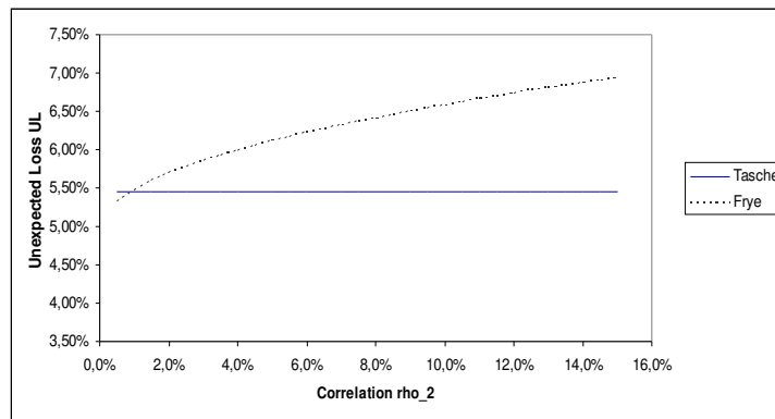
Figure 7. Comparison of the 99,9% unexpected loss in the Tasche model and Frye model depending on \rho_2 (with p_H = 1\% , \mu = 45\% , \sigma = 15\% , \rho = 15\% , p_{cure} = 0\% )
