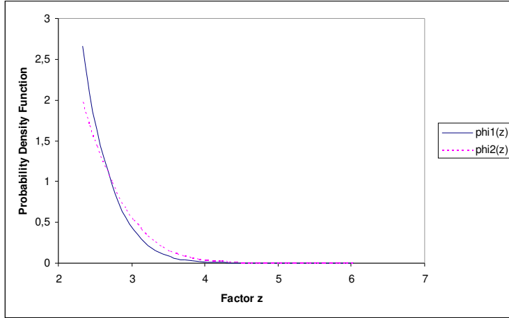
Figure 3. Density functions \phi_1 and \phi_2
