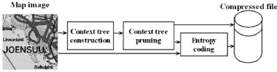
Fig. 2. Overall scheme of the proposed algorithm.
