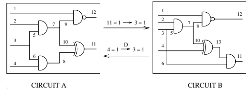
Figure 7: IB Transformations for Example 3.1
