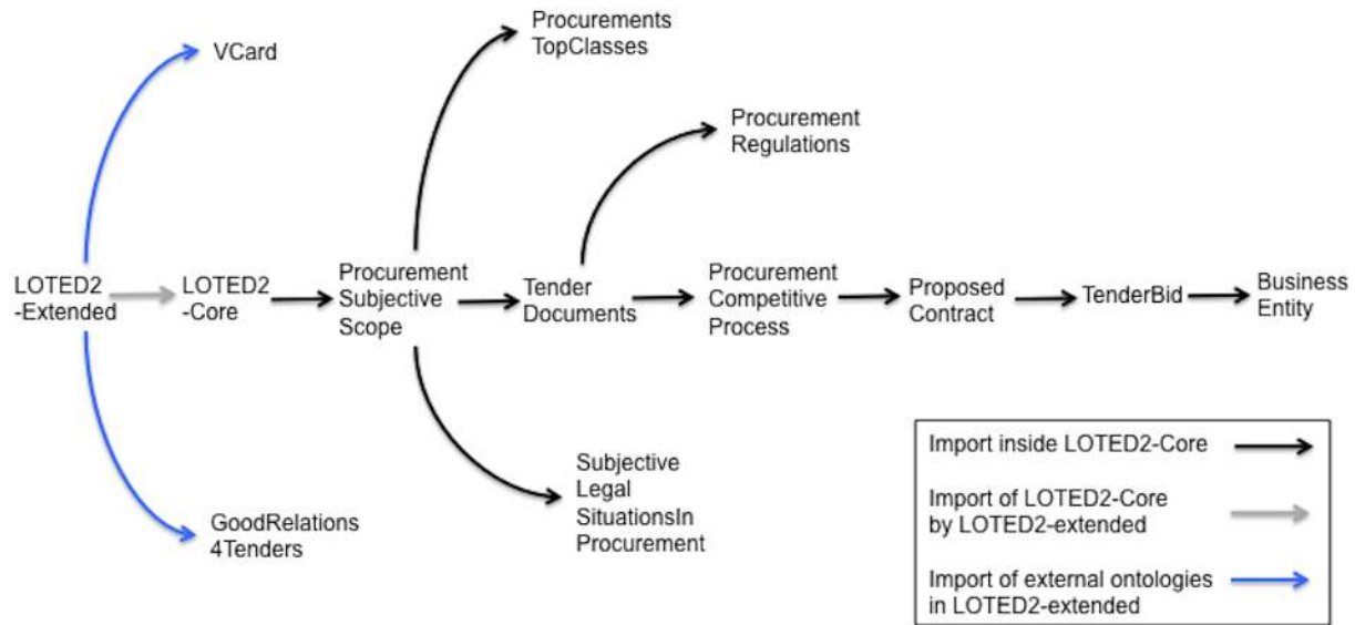
Fig. 3. Dependencies between LOTED2-core modules and external ontologies (GoodRelations4Tenders and VCard) in LOTED2-extended
