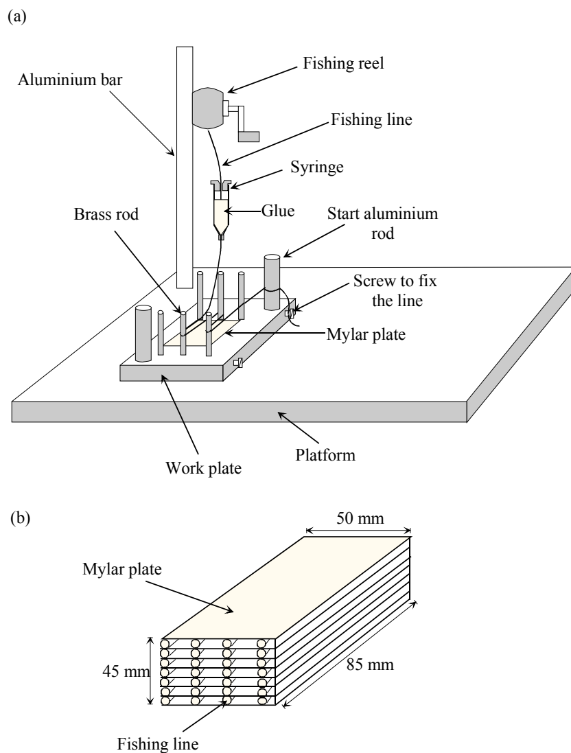
Figure 7.8: Illustration of the manufacturing technique of the parallel-plate stack. A plate is placed between the brass rods, then the glue coated fishing line coming from the syringe is wound around the rods to get parallel strings. The strings are then pressed onto the plate and an other plate may be placed. The procedure is repeated until the needed height of the stack is reached. a) Setup. b) A parallel plate stack as released from the work plate.
