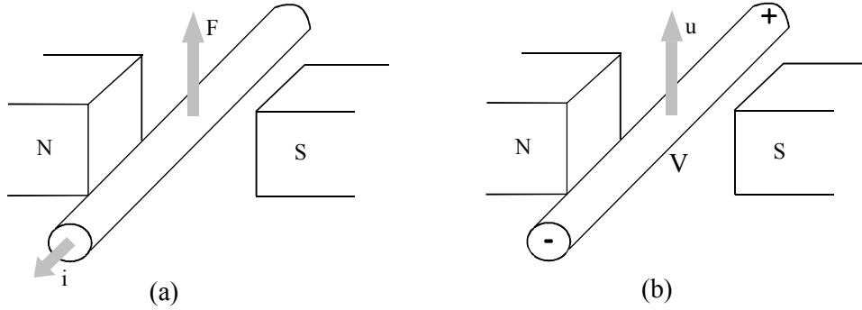
Figure 5.3: Illustration of the Lorentz force and Faraday's law. (a) A current i flowing through a conductor, placed in a magnetic field, produces a force F on the conductor. (b) The velocity u of a conductor in a magnetic field induces a voltage V across the conductor.
