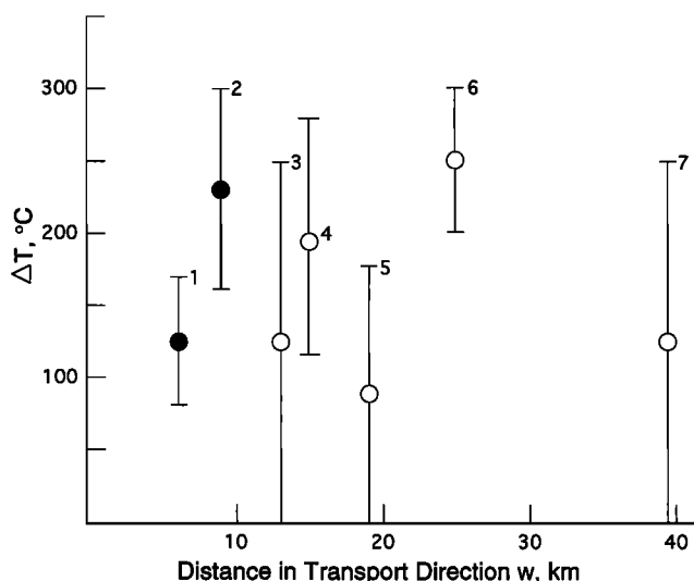
Figure 5. Maximum variation of paleotemperature in down-dip direction across footwalls of Cordilleran detachments, just prior to unroofing. Solid symbols indicate upper crustal sections only. Locations and sources: 1, Piute Mountains detachment, eastern Mojave Desert, California [Foster et al. , 1991]; 2, southwestern Harcuvar Mountains, west central Arizona [Richard et al. , 1990]; 3, Garden Wash detachment, South Virgin Mountains, Nevada [Fitzgerald et al. , 1991; Fryxell et al. , 1992; J. E. Fryxell, unpublished data 1994]; 4, Chemehuevi Mountains detachment, lower Colorado River trough, California [John and Foster, 1993]; 5, Newberry Mountains detachment, central Mojave Desert, California [Dokka, 1993]; 6, Amargosa detachment, Death Valley region, California [Holm and Wernicke, 1990; Holm et al. , 1992; Holm and Dokka, 1993]; 7, Buckskin-Rawhide detachment, lower Colorado River trough, Arizona [Richard et al. , 1990; Spencer and Reynolds, 1991].
