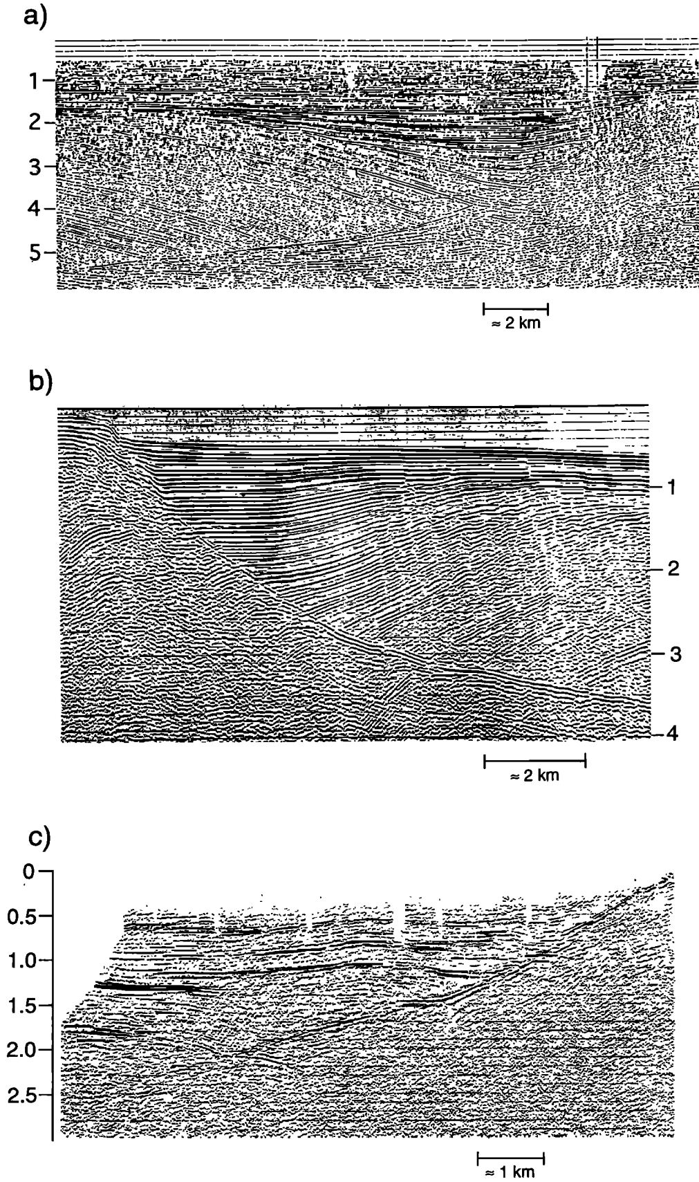
Figure 7. Seismic reflection profiles of low-angle normal faults. Vertical scales are all two-way travel times, in seconds. (a) Gulf of Bohai, east of Beijing, China, from Zhang [1994]; (b) Gulf of Oman, from Wernicke and Burchfiel [1982]; (c) Lamoille Valley, Nevada, from Smith et al. [1989]. See text for discussion.
