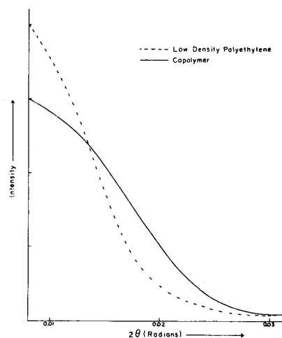
Figure 1. Angular dependence of low angle X-ray scattering pattern from low-density polyethylene and the un-ionized acid copolymer.
